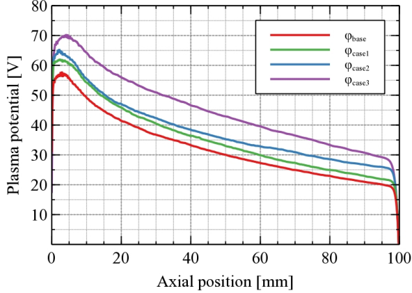
Figure 16. Plasma potential profiles.
