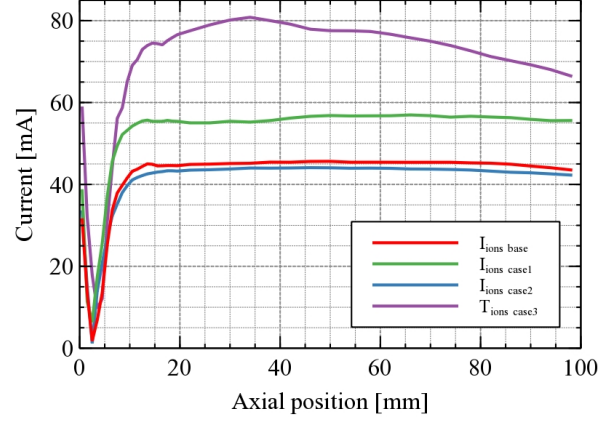
Figure 13. Ion currents.
