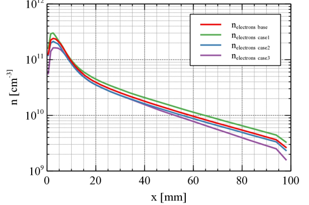
Figure 17. Density distributions.
