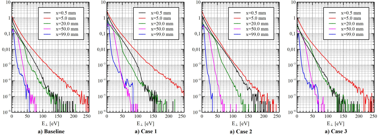
Figure 14. Electron energy distribution functions at different locations.
