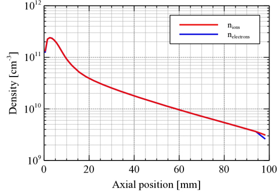
Figure 5. Density distribution.
