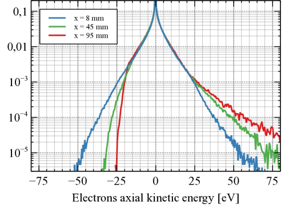
Figure 9. EEDF at different positions.
