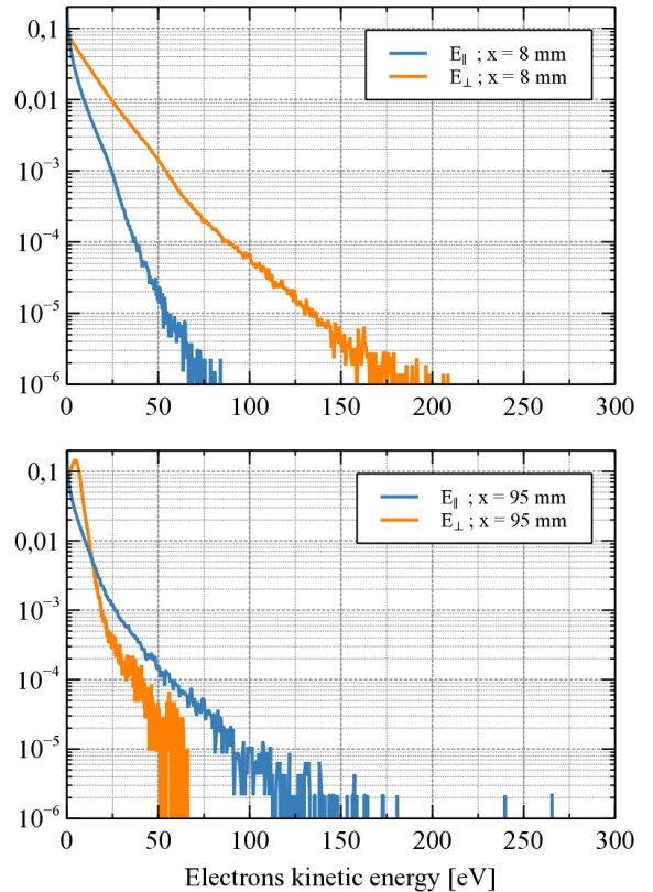
Figure 10. Perpendicular and parallel EEDF at two locations. Upper graph : in the source. Lower graph: close to the domain outlet.
