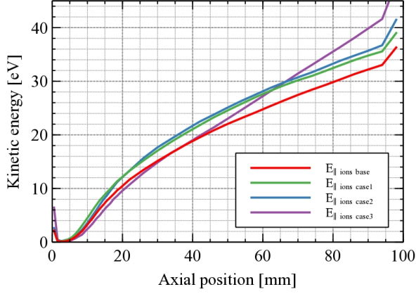
Figure 12. Ion mean kinetic energies.
