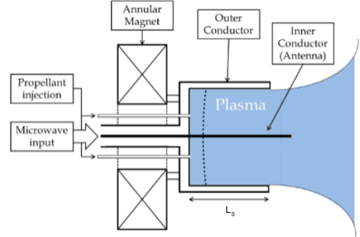
Figure 1. Schematic view of the ECRA thruster under development at Onera. 6
