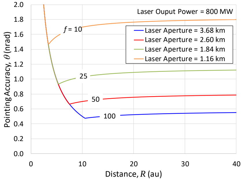
Figure 8. Example for required laser pointing accuracy that varies from 1.5 to 0.5 nrad for amplification factors from 10 to 100.
