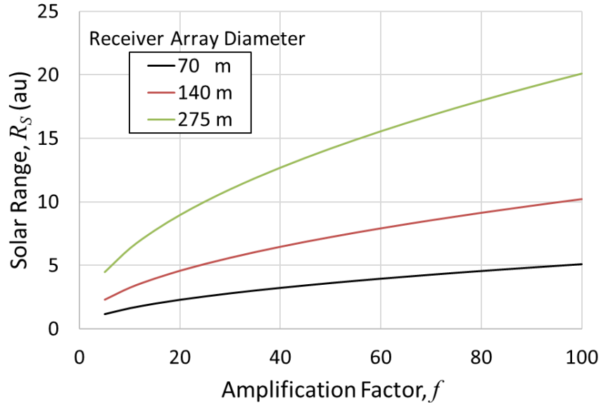
Figure 4. Solar range at which operation at the maximum EP system power can be sustained for three sizes of the PV array on the LEV. For an amplification factor of 100, full power operation at 10 MW could be maintained at 5 au (Jupiter) with a 70-m PV receiver array, 10 au (Saturn) with a 140-m array, and 20 au (Uranus) with a 275-m array.
