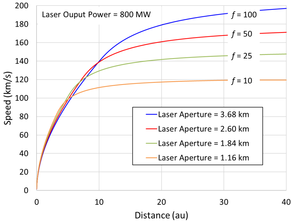
Figure 3. Amplification factors, f , of between 10 and 100 with a laser output power of 800 MW at 1064 nm are required to achieve final spacecraft speeds of between 100 and 200 km/s.
