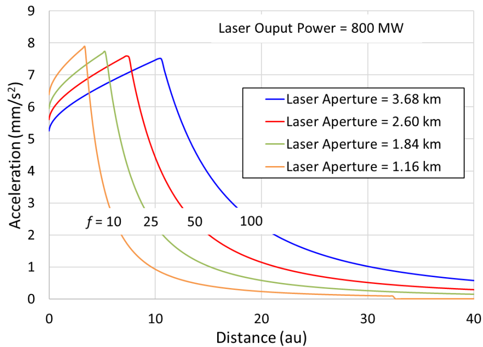
Figure 5. Example: LEV accelerations peak at between 7 and 8 mm/s 2 and then decrease at larger ranges as the laser beam spreads out and the LEV's photovoltaic array intercepts a smaller fraction of the beamed power.
