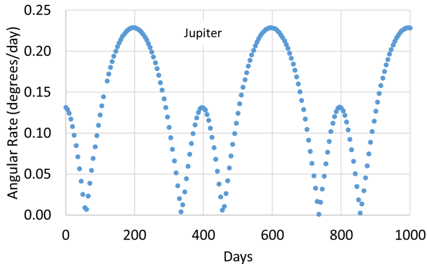
Figure 7. Angular rate required of the transmit laser vehicle to point continuously at an LEV at Jupiter.
