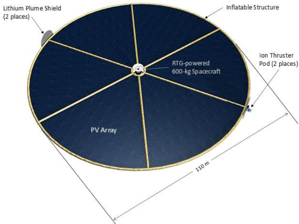
Fig. 11. Configuration of the Laser-powered, Electrically-propelled Vehicle (LEV). The vehicle includes a 110-m-diameter photovoltaic array for receiving the beamed laser power, a 10-MW lithium-fueled ion propulsion system that produces a specific impulse of 40,000 s, and a 600-kg RTG-power spacecraft located at the center of the PV array.
