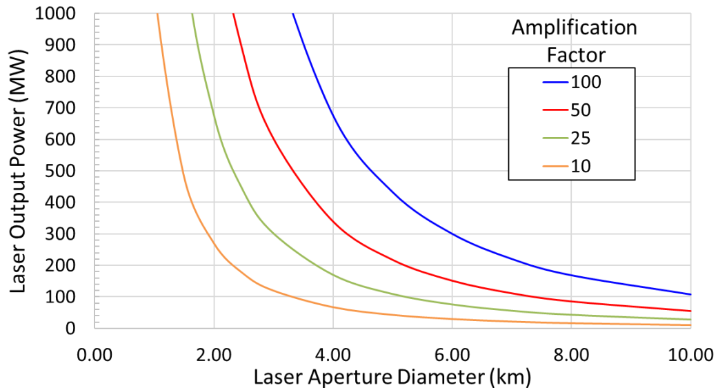
Figure 2. Plot of Eq. (6) showing that a very large, very high power laser is required to significantly increase the power density of photons relatively to solar insolation (for a laser wavelength of 1064 nm).
