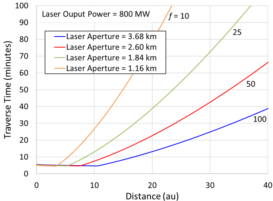
Fig. 13. Example estimates for the time it takes for the LEV to traverse (starting at rest) from the edge of the power beam to the center assuming 100% of the thrust is allocated to this traverse.
