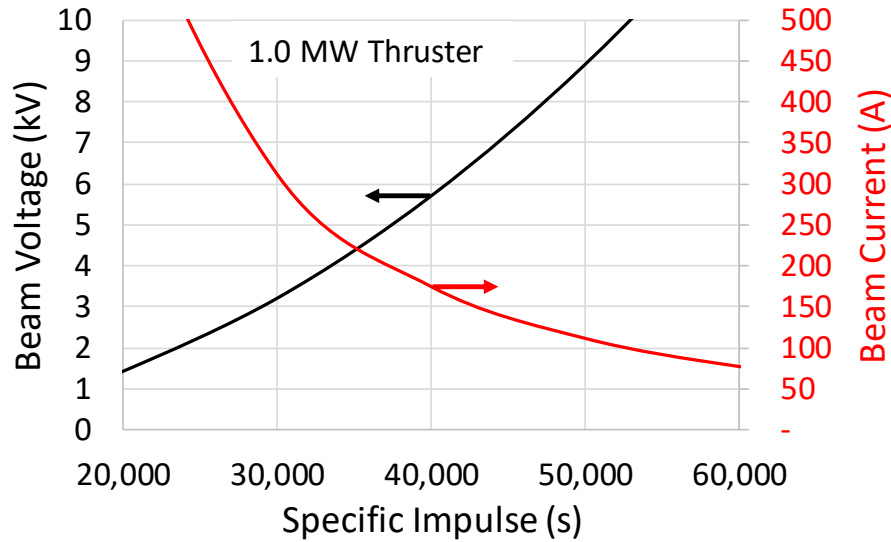
Figure 10. A 1.0-MW, lithium-fueled, gridded ion thruster operating at a specific impulse of 40,000 s would require a beam current of 175 A. While this is much higher than state of the art ion thrusters, the ability to cryopump the lithium exhaust at room temperature makes testing such a thruster feasible.
