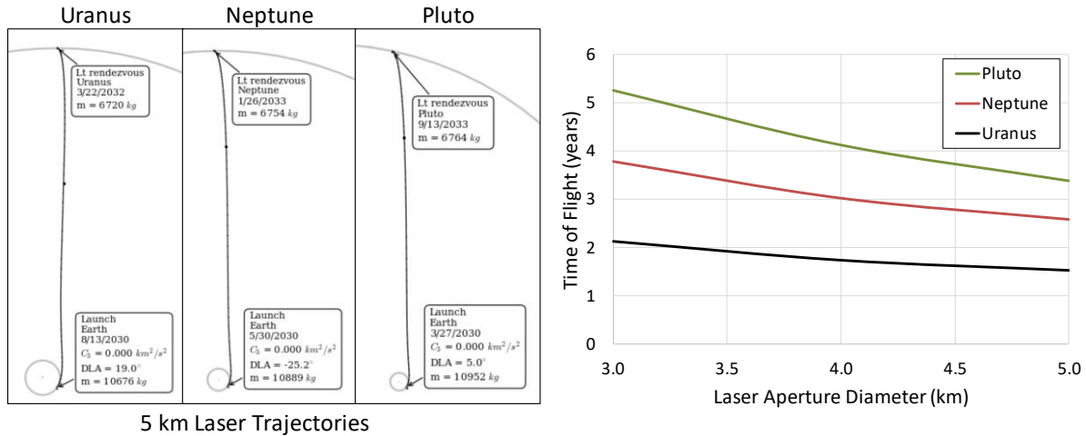
Figure 14 Short flight times for robotic rendezvous missions to the outer planets require \Delta V 's of approximately 170 km/s and are potentially enabled with the Direct-Energy Electric Propulsion system architecture. The mission performance indicated in this figure requires an 800 MW output power laser at a wavelength of 1064 nm with aperture diameters between 3 and 5 km to power an LEV with a 10 MW direct-drive electric propulsion system operating at a specific impulse of 40,000 s.
