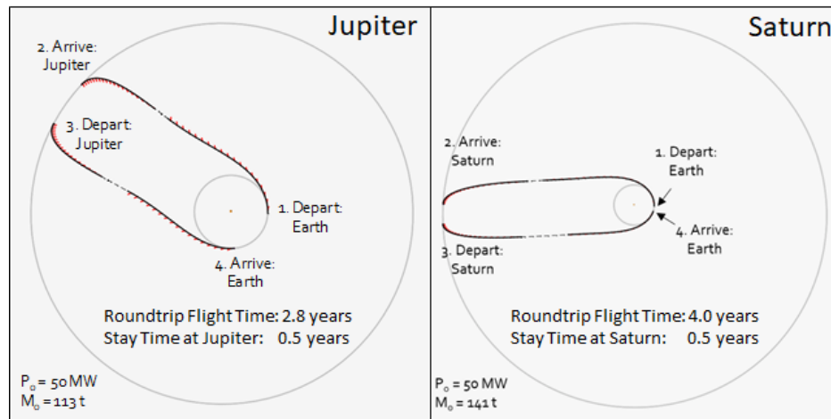
Figure 15 Human-scale missions to Jupiter and Saturn with reasonable roundtrip flight times may be enabled by the Direct-Energy Electric Propulsion (DEEP) system architecture.
