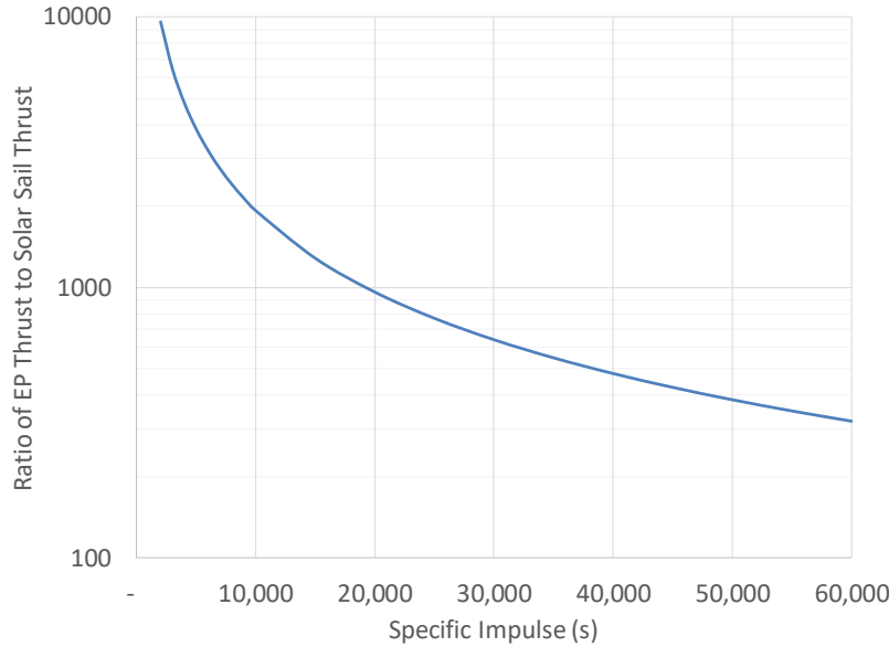
Figure 16. At a specific impulse of 40,000 s, an electric propulsion based vehicle produces approximately 500 times the thrust of a laser-propelled sail for the same laser power.
