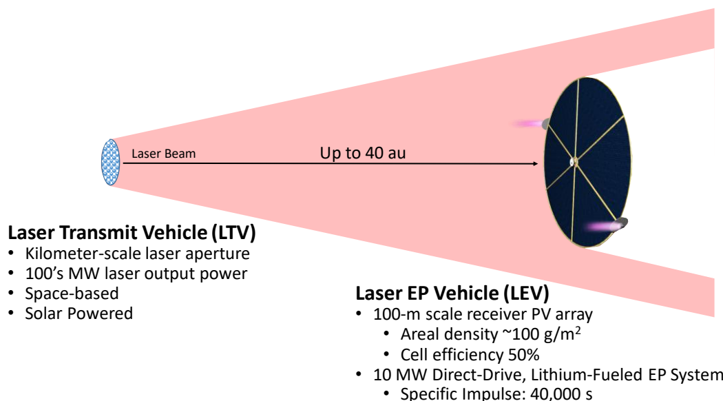
Figure 1. Depiction of a Directed-Energy Electric Propulsion (DEEP) propulsion architecture potentially capable of enabling missions with characteristic velocities of between 100 and 200 km/s. The architecture consists of a laser transmit vehicle (LTV) that is a high-power, large-aperture, space-based laser transmitter, and a laser electric propulsion vehicle (LEV) that collects a fraction of the laser power to operate an ultra-high specific impulse electric propulsion system.
