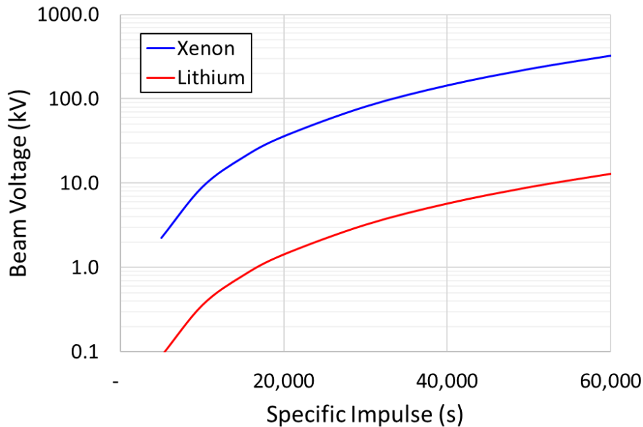
Figure 9. The use of lithium instead of xenon enables gridded ion thruster operation at a specific impulses in the range 40,000 to 60,000 s with beam voltages of 6 to 12 kV. The corresponding beam voltages with xenon would be 140 to 320 kV.
