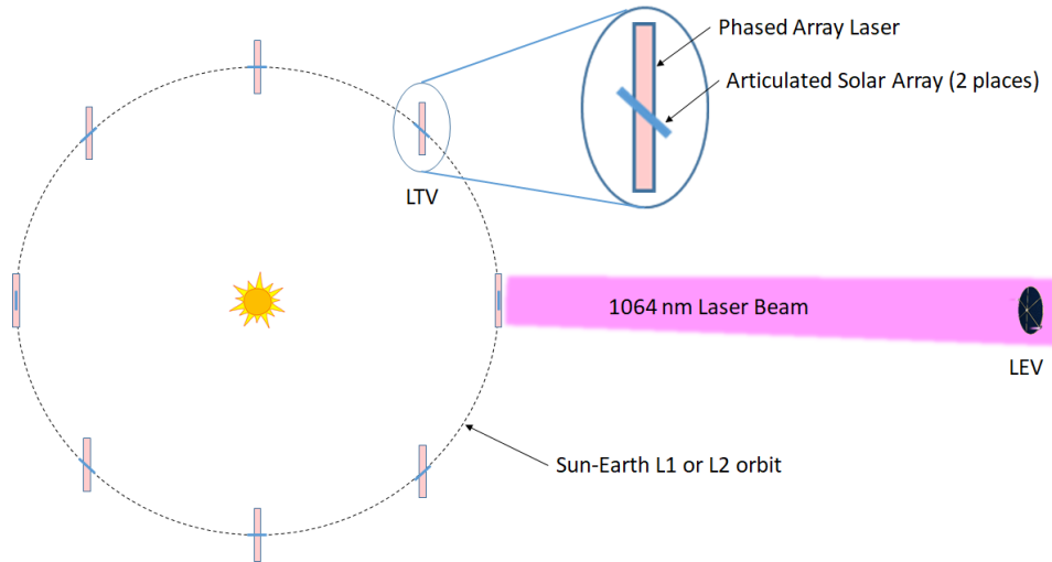
Figure 6. Illustration of the transmit laser at Sun-Earth L1/L2 indicating that the solar array that powers the transmit laser must articulate completely around once per year while the laser remains locked on to the LEV.
