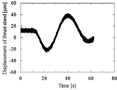
Figure 4. Thrust waveform with nylon target. UV-LED was irradiated to the target surface between 10 s and 14 s
