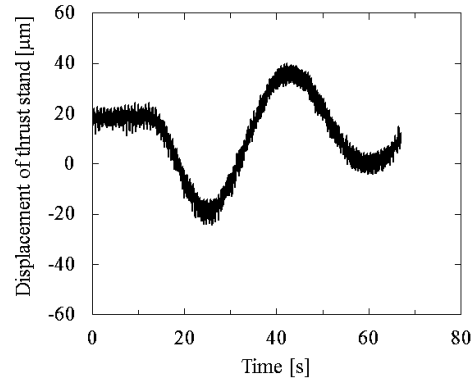
Figure 5. Calibration waveform with electrostatic actuator. Applied voltage = 30 V
