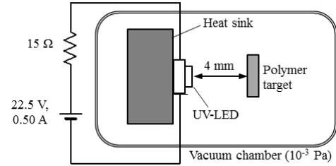
Figure 2. Schematic of experimental setup for mass consumption rate measurement.
