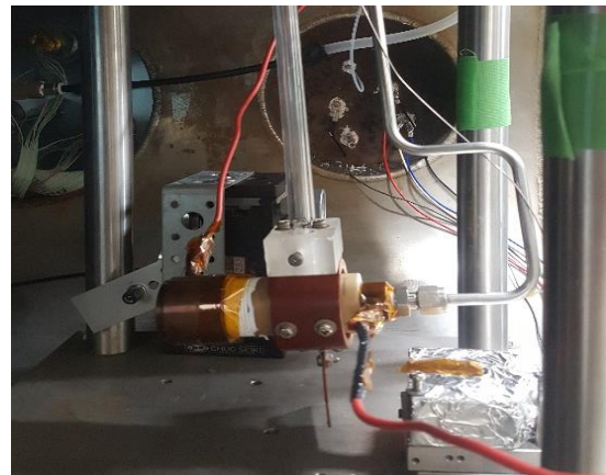
Figure 6. Photo of An Arcjet with Thrust Stand.
