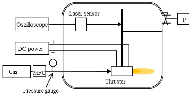
Figure 3. Experimental setup.
