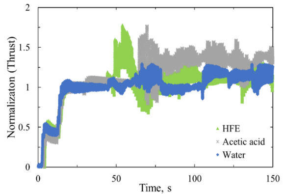
Figure 9. Results of normalization thrust for various propellants.
