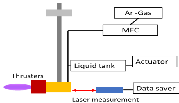
Figure 4. Schematic of Calibration method.
