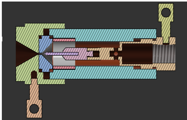
Figure 5. Cross section of Arcjet Thruster
