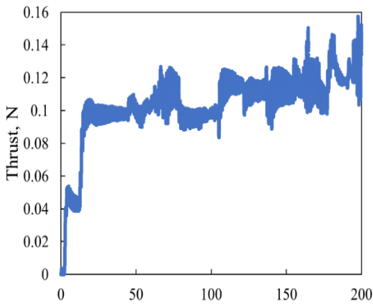
Figure 8. Results of thrust (At water 8 mg/s).
