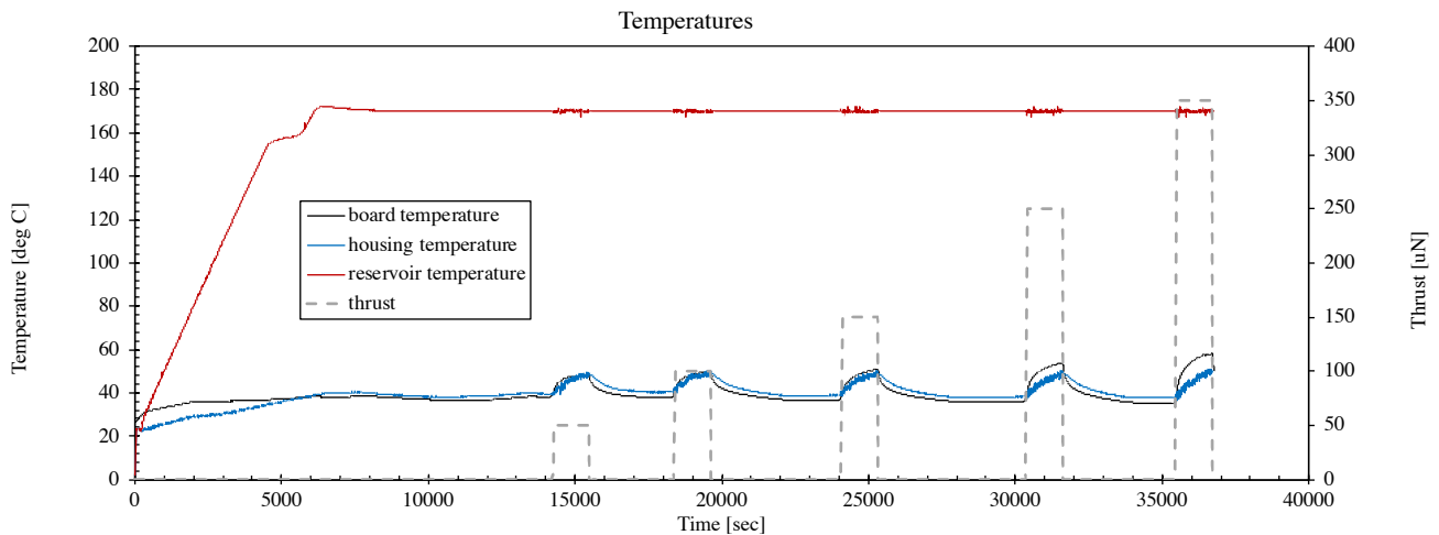
Figure 5. IFM06.03 Thruster temperature telemetry during multiple consecutive firings with different thrust levels
