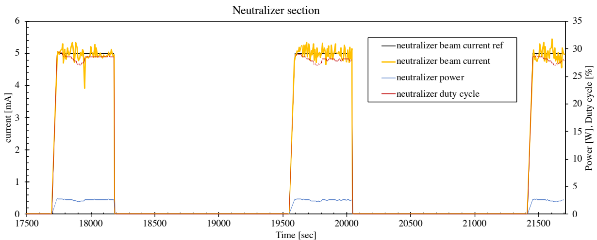
Figure 10. IFM06.02 Neutralizer telemetry during multiple consecutive firings
