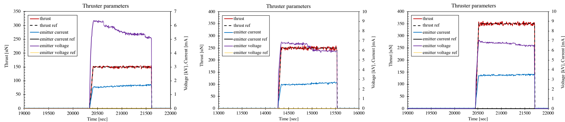
Figure 13. IFM06.04: Thrust-controlled firing of thruster, 150 \mu\text{N} (left), 250 \mu\text{N} (center) 350 \mu\text{N} (right)
