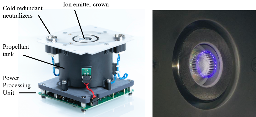
Figure 2. IFM Nano Thruster (left), IFM crown emitter during ion emission (right, from Ref. 10)
