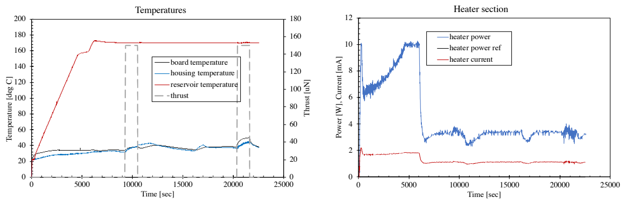
Figure 7. IFM06.04 Thruster temperature telemetry (left) and heater power (right) during multiple consecutive firings
