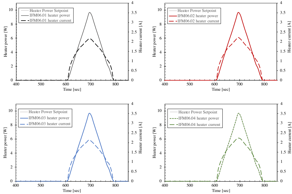
Figure 4. Heater section commissioning for IFM06.01, IFM06.02, IFM06.03 and IFM06.04 showing good repeatability between thrusters
