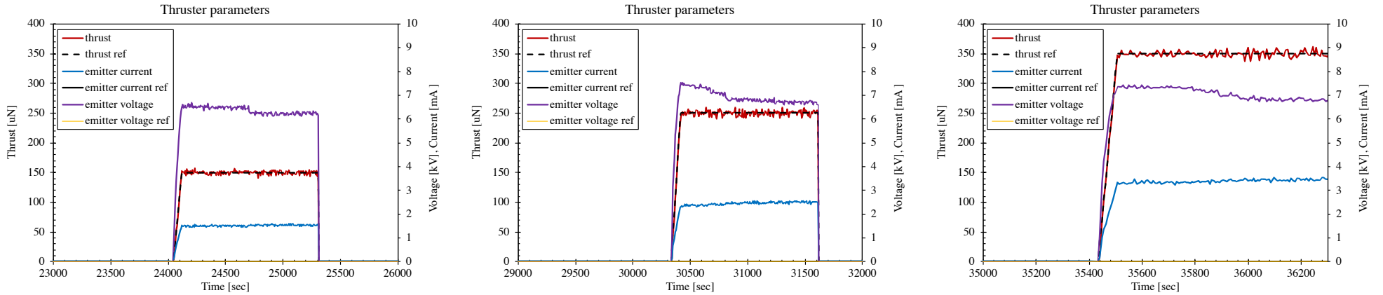
Figure 12 IFM06.03. Thrust-controlled firing of thruster, commanded thrust levels: 150μN (left), 250μN (center) 350μN (right), transient detail shown
