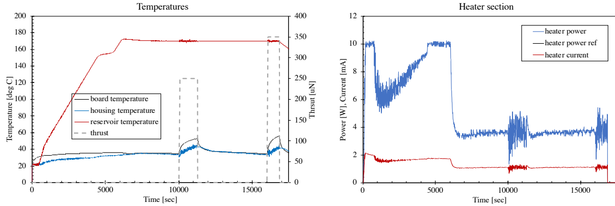
Figure 6. IFM06.01 Thruster temperature telemetry (left) and heater power (right) during multiple consecutive firings
