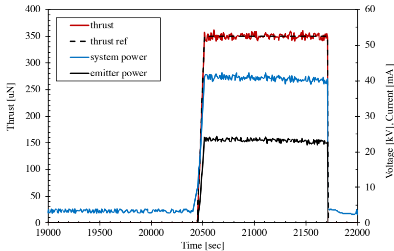
Figure 14. IFM06.04: System power consumption and emitter power draw for 350 \mu N operation point
