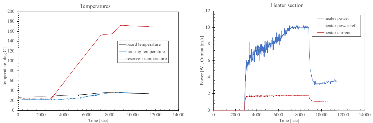
Figure 8. IFM06.02 Thruster temperature telemetry (left) and heater power (right) during transition from cold state to hot standby state
