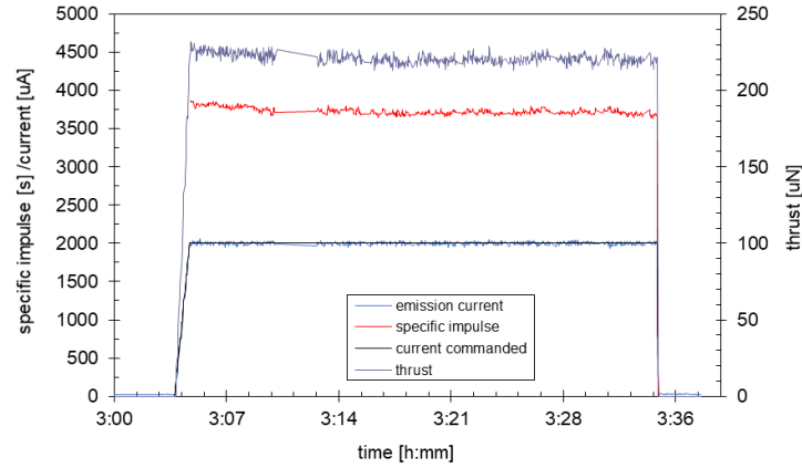
Figure 3. 30min IOD firing for independent orbit change verification 10
