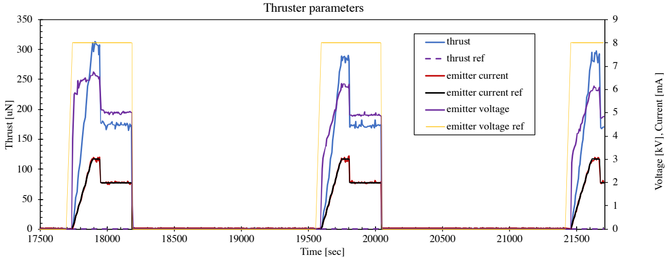
Figure 9. IFM06.02 Thruster telemetry during multiple consecutive firings
