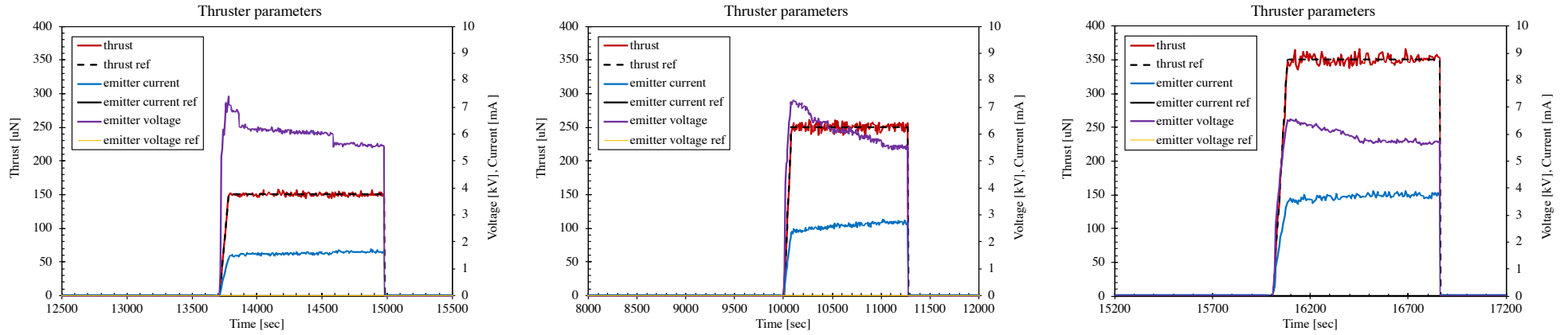
Figure 11. IFM06.01: Thrust-controlled firing of thruster, 150μN (left), 250μN (center) 350μN (right)
