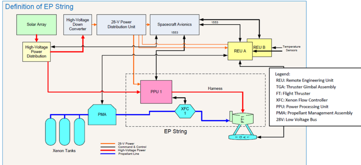
Figure 3. AEPS string EP string definition, Ref. [8].
