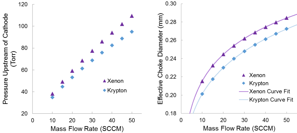
Figure 4. Propellant gas pressure upstream of a room temperature hollow cathode as a function of propellant mass flow rate (left), and the effective choked orifice diameter for each of these data points (right).
