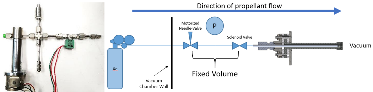
Figure 2. Photo (left) and schematic (right) of an experimental fixed-volume release system that can be used to provide an elevated propellant mass flow rate during heaterless hollow cathode ignition without using a mass-flow controller.
