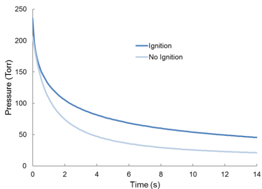
Figure 9. Comparison of propellant pressure in a fixed-volume release with and without an ignition performed.
