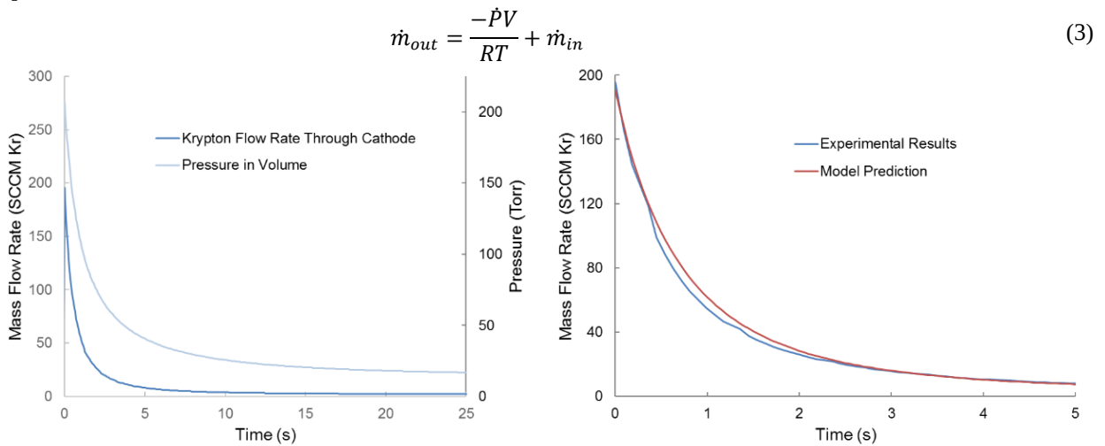
Figure 6. Curve-fit of experimentally measured fixed-volume pressure, and calculated flow rate (Eq. (3)) as a function of time (left), and comparison of experimental results and flow model (right). Time t = 0 corresponds to the valve opening, releasing approximately 13 mg of krypton propellant from a 13 cm 3 volume.
