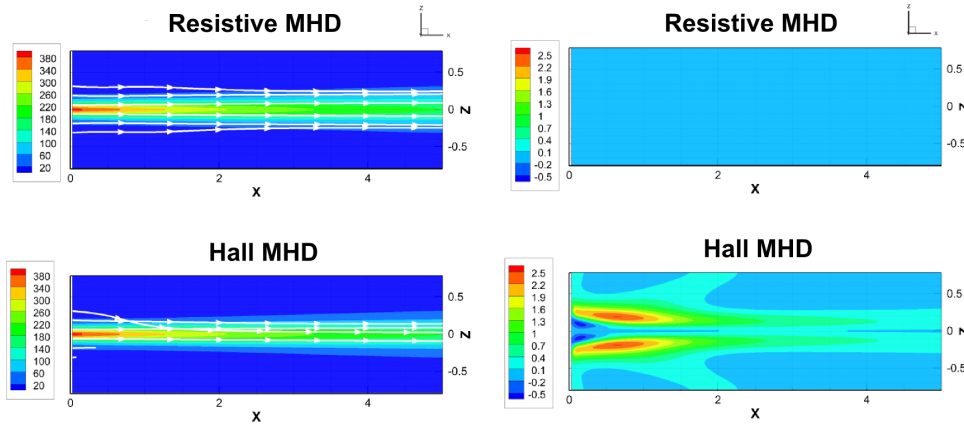
Figure 8. Left: Contours of axial velocity and velocity streamlines, Right: Contours of azimuthal ( \hat{\theta} ) velocity (m/s)
