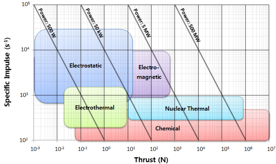
Figure 1. Specific impulse and thrust operating regimes for space propulsion methods with power level contours.
