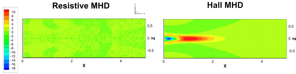
Figure 7. Contours of axial ( \hat{x} ) current
