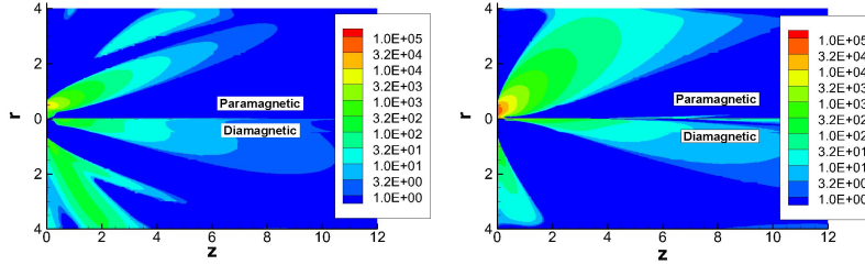
Figure 6. Induced currents, J (A/m 2 ), in \hat{\theta} direction. Top half contours are paramagnetic (positive \hat{\theta} ) and bottom half contours are diamagnetic (negative \hat{\theta} ).
