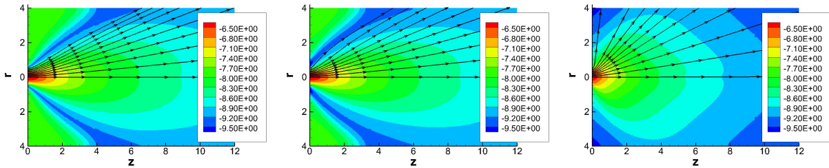
Figure 3. Density contours ( \log_{10}(kg/m^3) ) with velocity stream lines. Left: No magnetic field, Center: B_0 = 0.002 (T), Right: B_0 = 0.02 (T)
