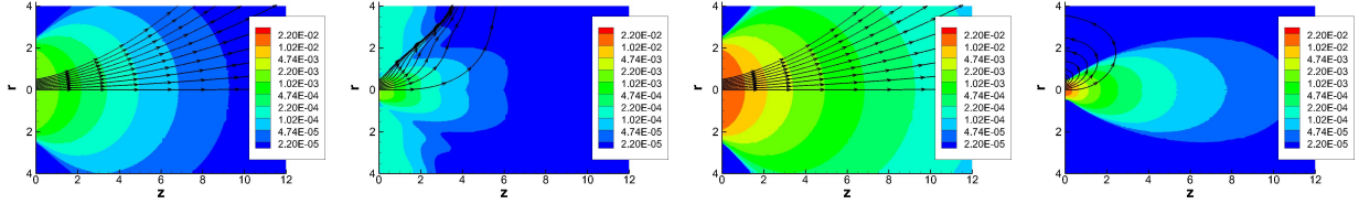
Figure 5. Axial magnetic field contours with magnetic field streamlines. First: Initial magnetic field for B_0 = 0.002 (T), Second: Final magnetic field for B_0 = 0.002 (T), Third: Initial magnetic field for B_0 = 0.02 (T), Fourth: Final magnetic field for B_0 = 0.02 (T)
