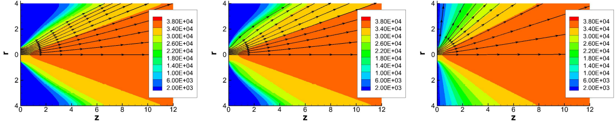
Figure 4. Axial velocity contours (m/s) with velocity streamlines. Left: No magnetic field, Center: B_0 = 0.002 (T), Right: B_0 = 0.02 (T)
