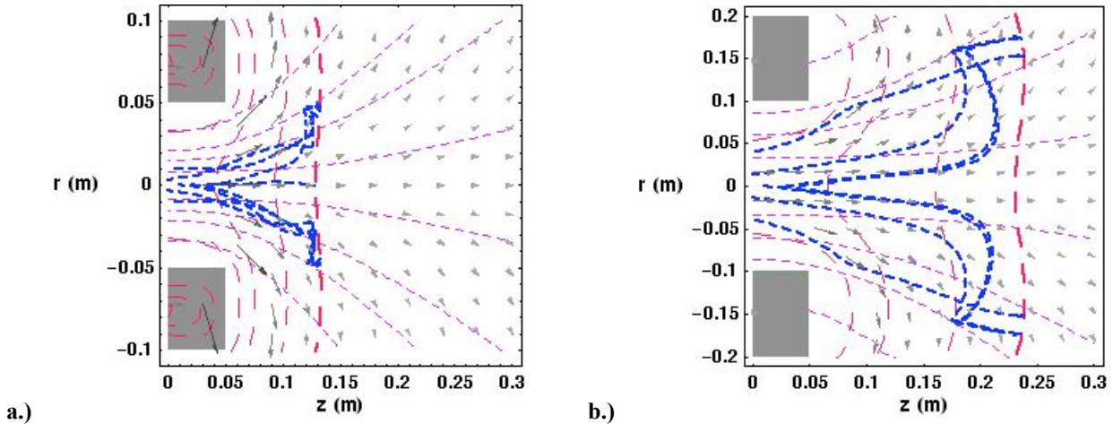
Figure 6. Ray paths of helicon-ECR waves in helicon source overlaid on magnetic field vectors and contours, and density contours. a.) Narrow source. b.) Broad source.
