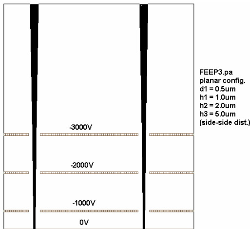
Figure 3: Two small vias shown extracting and accelerating either nano-particle or ions (likely separate vias for each kind).
