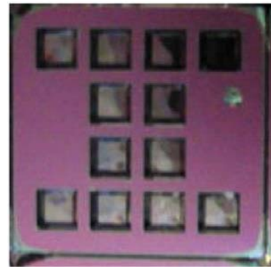
Figure 10: First-generation MEMS gate design showing the viewing windows etched into the bulk silicon. Each viewing window contains tens of thousands of emission channels. The current MEMS gate is a second-generation design.
