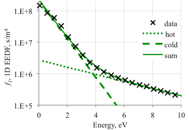
Figure 6. Planar Langmuir probe analysis. Measurements are performed using the first derivative of the electron current to obtain the 1D EEDF and least-squares fitted Maxwellians.
