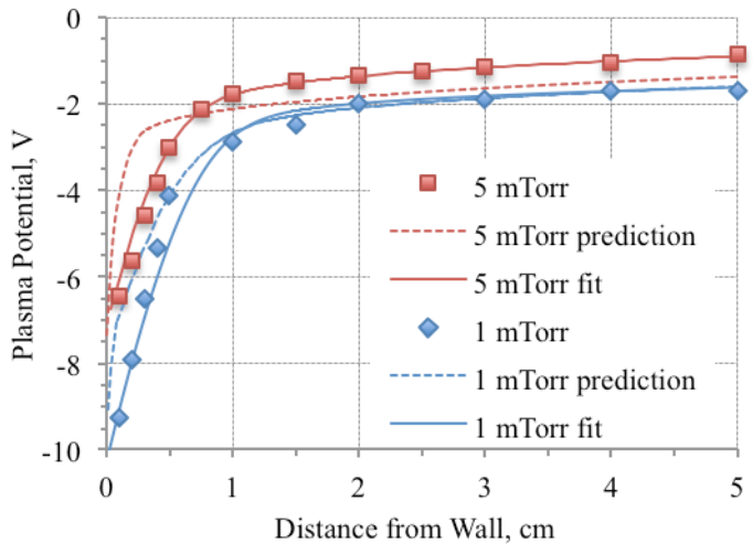
Figure 5. Measured potential profiles compared to fluid asymptotic matching theory.
