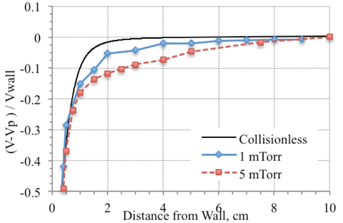
Figure 4. Measured sheath potential profiles normalized by wall potential. Collisionless theory added for comparison.
