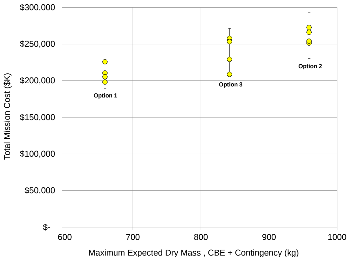
Figure. 5. Estimated total mission costs (Phases A-E) in FY'13$ for a class D, single-string, technology demonstration mission based on the options listed in Table 3.
