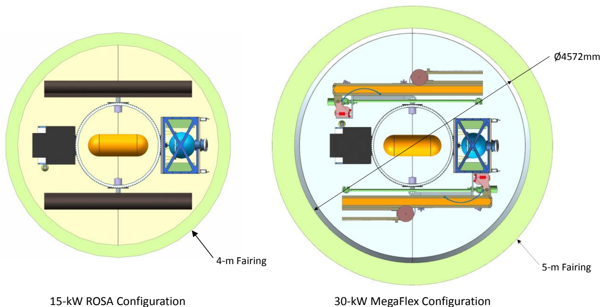
Figure 2. Option 1 (left) shown inside a 4-m launch vehicle fairing and Options 2 & 3 shown inside a 5-m fairing.
