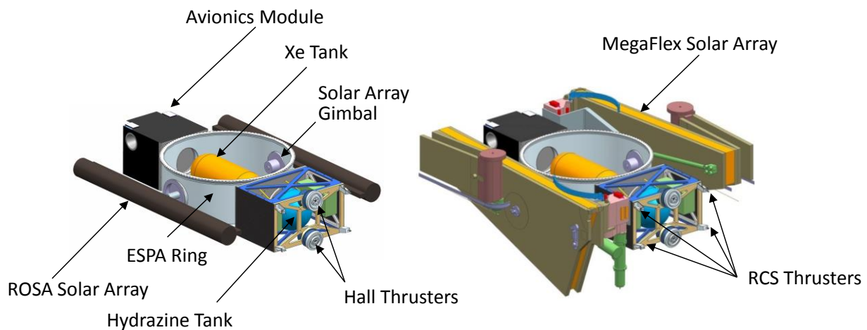
Figure 1. Stowed configurations for Option 1 (left) and Options 2 & 3 (right) with a standard ESPA ring.
