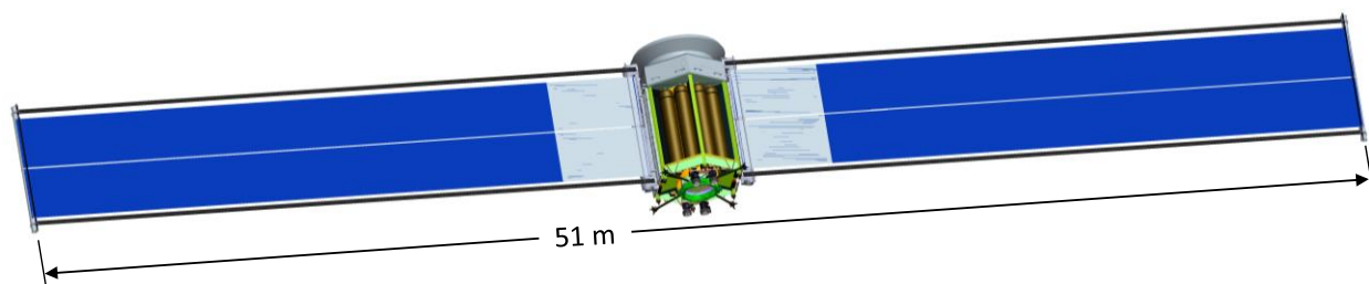
Figure 6. ARV flight configuration pictured with ROSA solar arrays.
