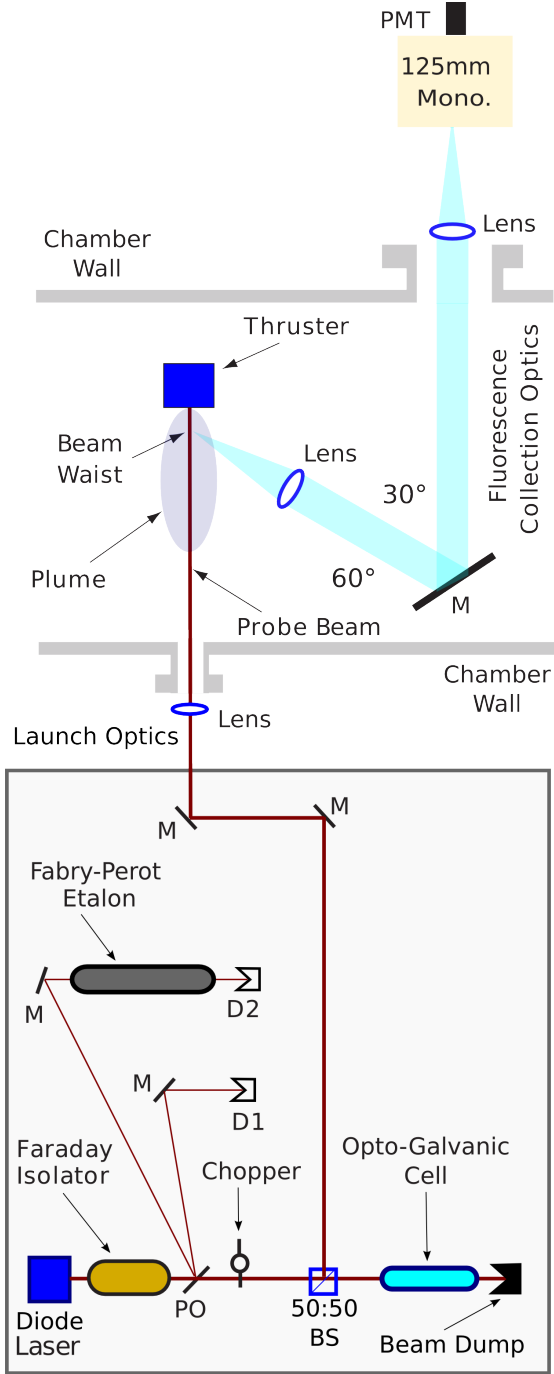
Fig. 2 Layout of Kr II laser-induced fluorescence apparatus showing all relevant optical components, portions of the vacuum chamber, and Hall effect thruster plume.
