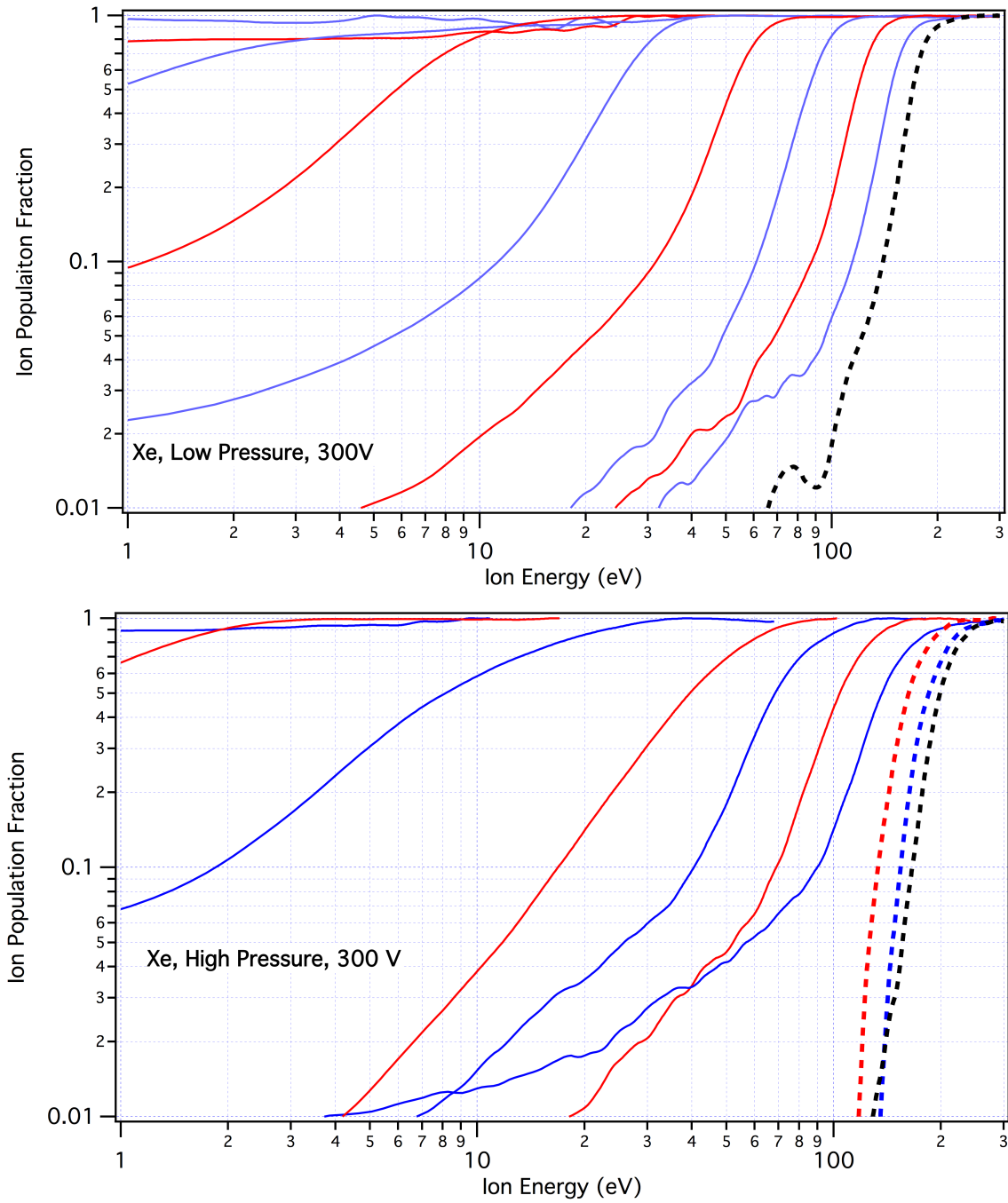
Fig. 11 Integrated xenon ion energy distributions calculated from xenon velocity distributions for the 300 V discharge potential case from Nakles and Hargus. 1 The exit plane is denoted by the black line and subsequent axial locations are noted by their axial position. Note the dashed lines are used to denote populations with greater than typical noise in the fluorescence signal that may have masked the behavior of population fractions of less than 0.1.
