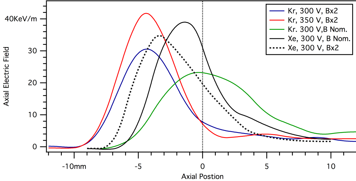
Fig. 5 Effective electric fields calculated from most probable velocity profiles for xenon, krypton at various operating condition. The nominal krypton magnetic field (B Nominal) electric field data 23 and xenon electric field data 1,13 are from previous publications.
