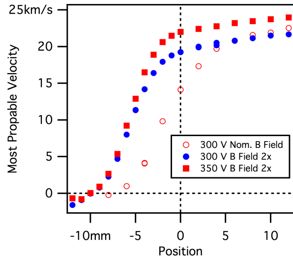
Fig. 4 Most probable axial Kr II velocities for three cases. Open circles represent nominal conditions from previous measurements. 23 Filled circles are for nominal conditions with 2\times applied magnetic field. Filled squares are likewise with an increased applied discharge potential (350 V vs. 300 V nominal).
