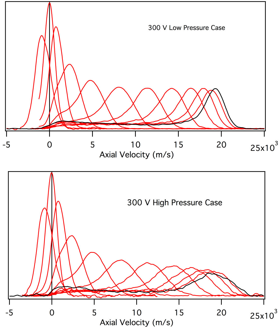
Fig. 7 Krypton ion (Kr II) velocity distributions for 300 V discharge potential at low background pressure (upper) and high background pressure (lower) ranging from the thruster exit plane (black trace at Z = 0 mm) to Z = -11 mm near the anode.
