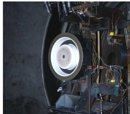
Figure 2. The NASA-300MS on a thrust stand.
