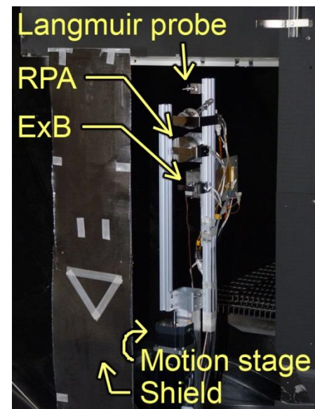
Figure 6. Photograph of the farfield probe tower.
