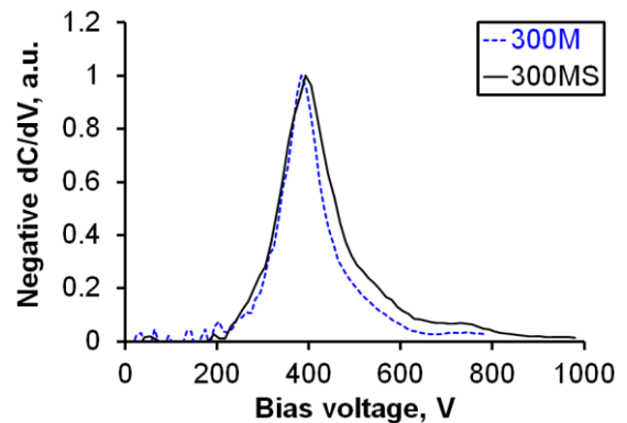
Figure 9. Comparison of ion energy-per-charge distributions for the 300M and 300MS at 400 V, 20 kW.
