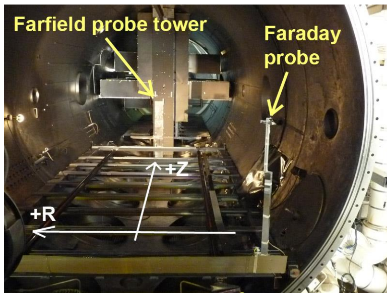
Figure 5. Photograph of the diagnostics setup.
