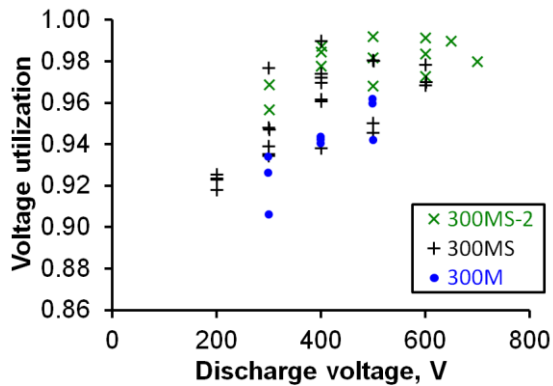
Figure 18. Voltage utilization efficiency as a function of the discharge voltage.
