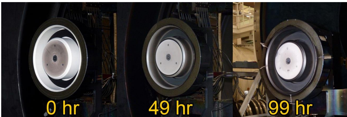
Figure 4. NASA-300MS prior to test (left), after 49 hours of testing (middle), and after 99 hours of testing (right).
