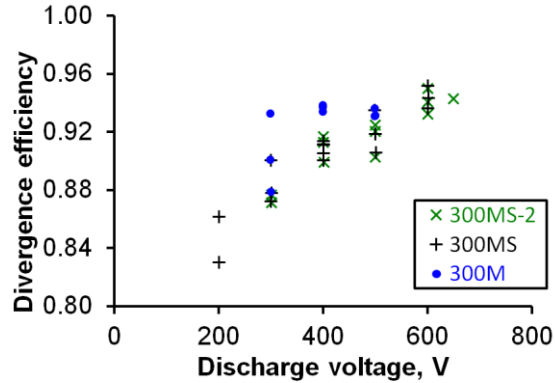
Figure 19. Divergence efficiency as a function of the discharge voltage.
