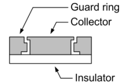
Figure 7. Diagram of the farfield Faraday probe.
