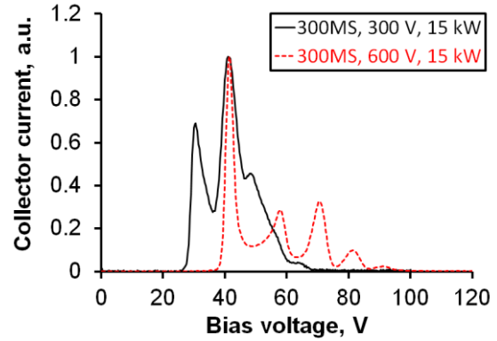
Figure 13. Comparison of ExB probe traces for the 300MS at 300 and 600 V, 15 kW.
