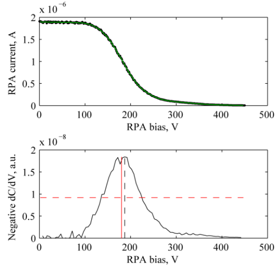
Figure 8. Sample RPA analysis plots.
