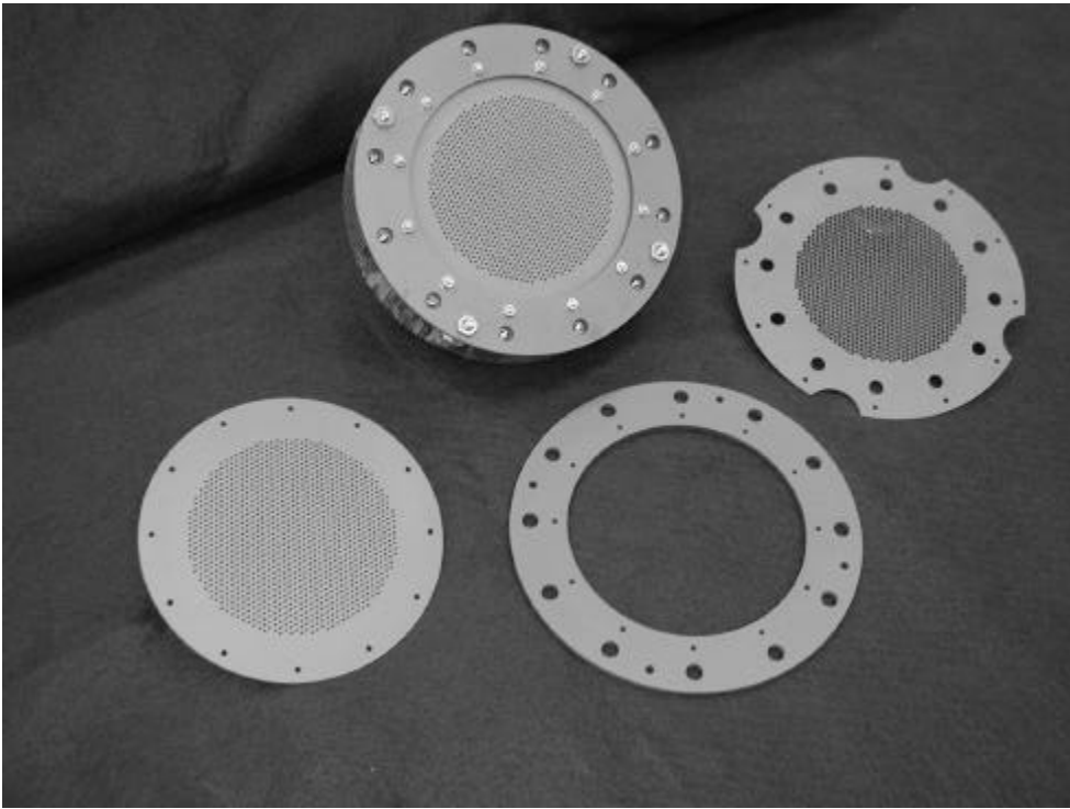
Figure 3. - 8 cm pyrolytic carbon grids, and carbon/carbon composite isolated mounting structure.
