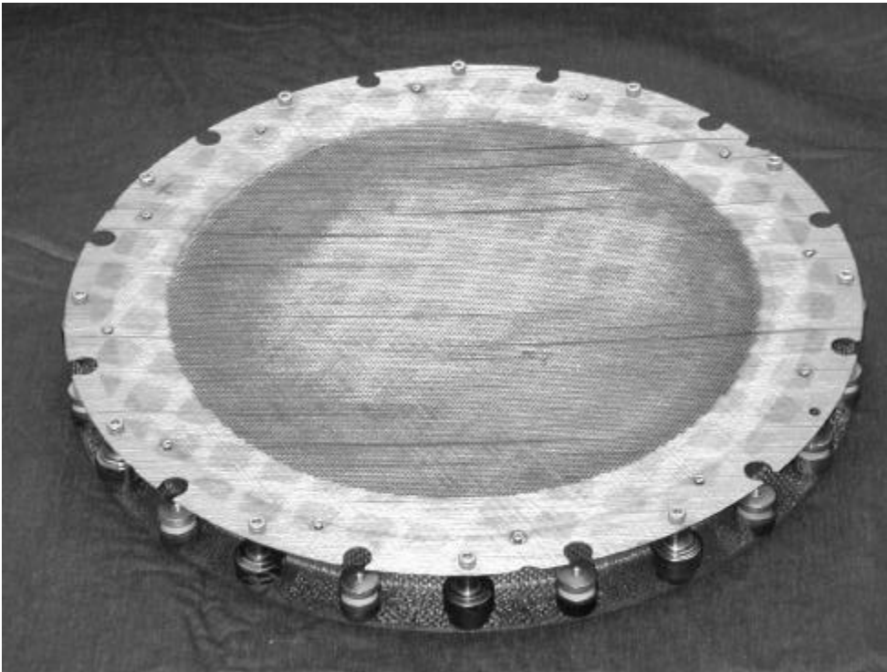
Figure 1. - 30 cm carbon/carbon composite ion optics assembly fabricated by JPL.
