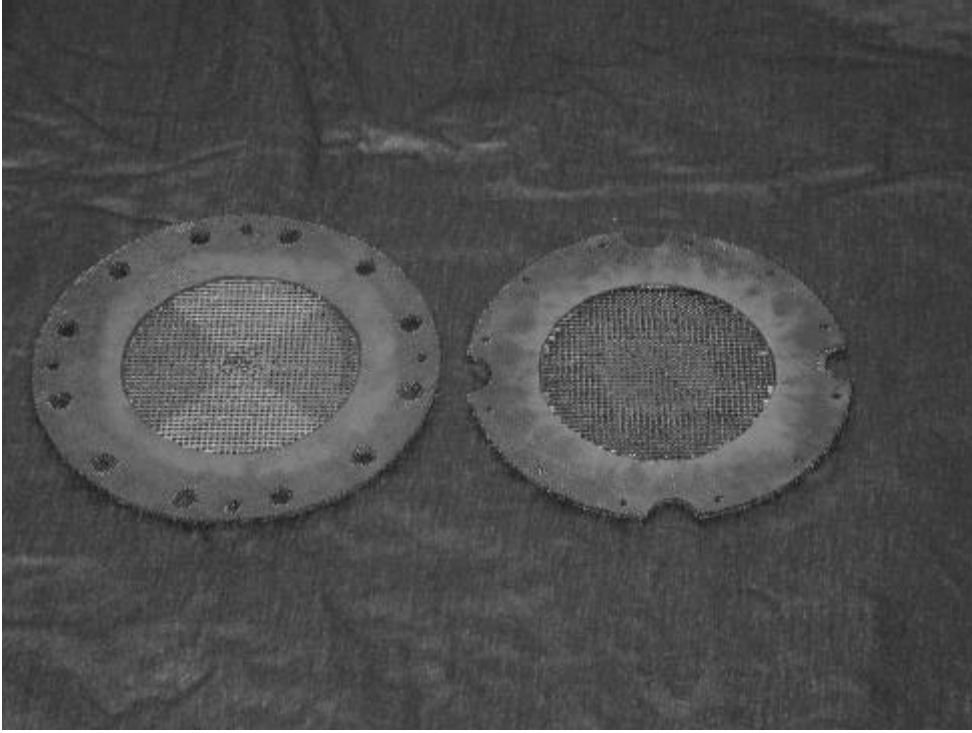
Figure 2. - 8 cm carbon/carbon composite accelerator and screen grids.
