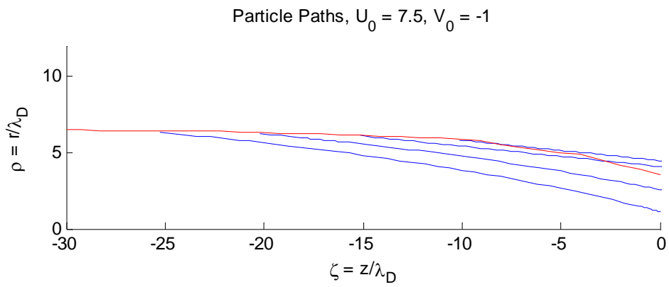
Figure 9 – Ion trajectories originating from four different starting points, U_0 = 7.5 .
