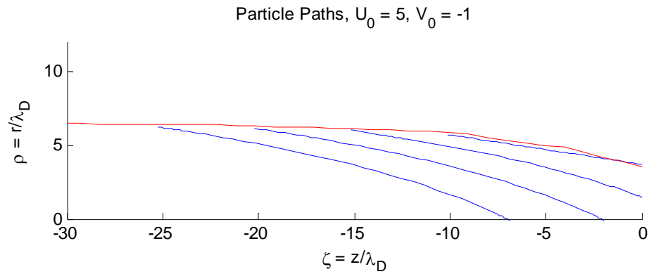
Figure 8 – Ion trajectories originating from four different starting points, U_0 = 5 .
