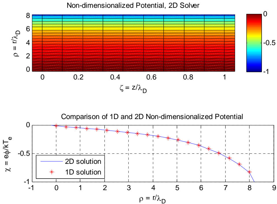
Figure 5 - 1D solution vs. 2D solver results, Example 2. In this case \chi = 0 at the outer boundary and \chi_w = -1 . The sheath thickness was 8.
