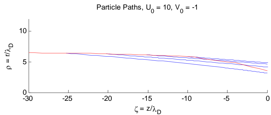
Figure 10 – Ion trajectories originating from four different starting points, U_0 = 10 .
