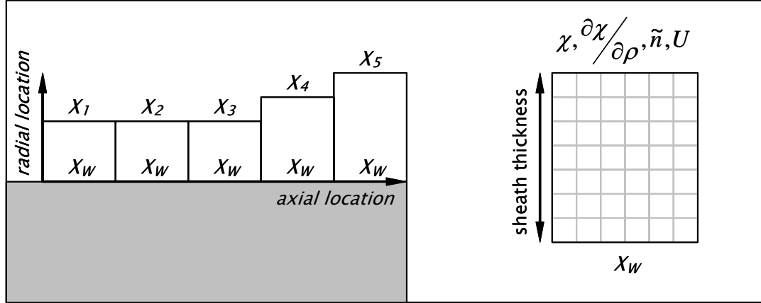
Figure 3 - Applying the 2D solver in a "quasi" 2D fashion. The solver was applied to cells over which the outer boundary values could be assumed constant.
