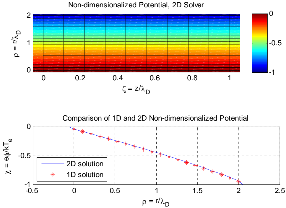
Figure 4 - 1D solution vs. 2D solver results, Example 1. In this case \chi = 0 at the outer boundary and \chi_w = -1 . The sheath thickness was 2.
