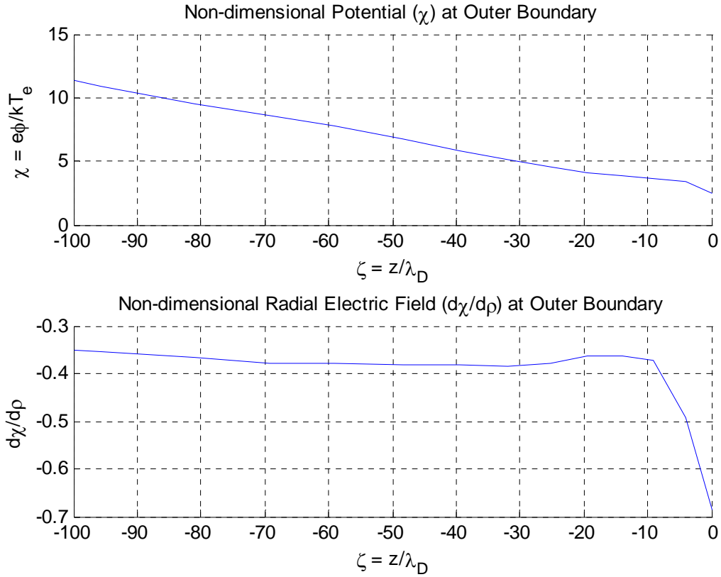
Figure 6 - Boundary conditions from the HPHall SPT-70 solution. Note that \zeta = 0 corresponds to the thruster exit plane.
