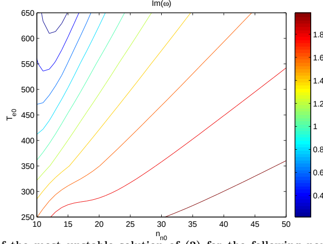
Figure 5. Growth rate of the most unstable solution of (2) for the following non-dimensional parameters: \tilde{k}_y = 0.25 , \tilde{v}_{ix0} = -5 , \tilde{v}_{nx0} = -5 , \tilde{\xi}_{i0} = 0.5 and \tilde{\xi}_{e0} = 0 . Parametric variation of \tilde{n}_{n0} and \tilde{T}_{e0}
