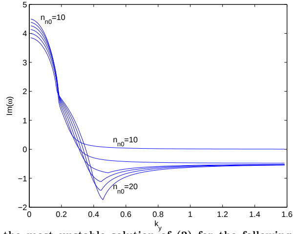
Figure 3. Growth rate of the most unstable solution of (2) for the following non-dimensional parameters: \tilde{v}_{ix0} = -5 , \tilde{v}_{nx0} = -5 , \tilde{\xi}_{i0} = 0.5 , \tilde{\xi}_{e0} = 0 and \tilde{T}_{e0} = 450 . Parametric variation of k_y and \tilde{n}_{n0}
