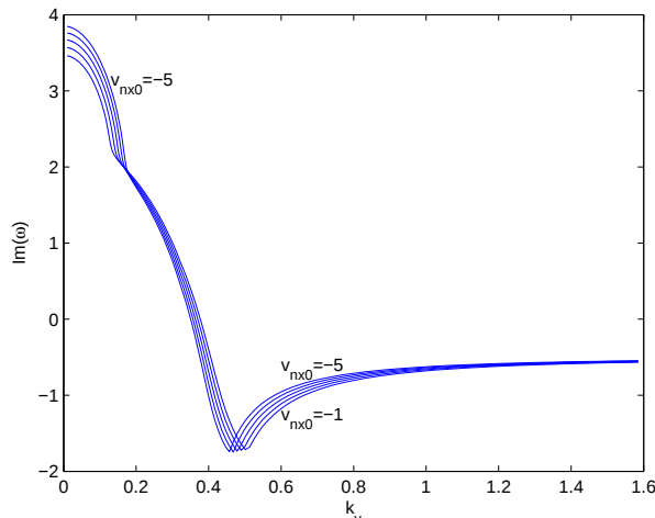
Figure 1. Growth rate of the most unstable solution of (2) for the following non-dimensional parameters: \tilde{n}_{n0} = 20 , \tilde{v}_{ix0} = -5 , \tilde{\xi}_{i0} = 0.5 , \tilde{\xi}_{e0} = 0 and \tilde{T}_{e0} = 450 . Parametric variation of \tilde{k}_y and \tilde{v}_{nx0}
