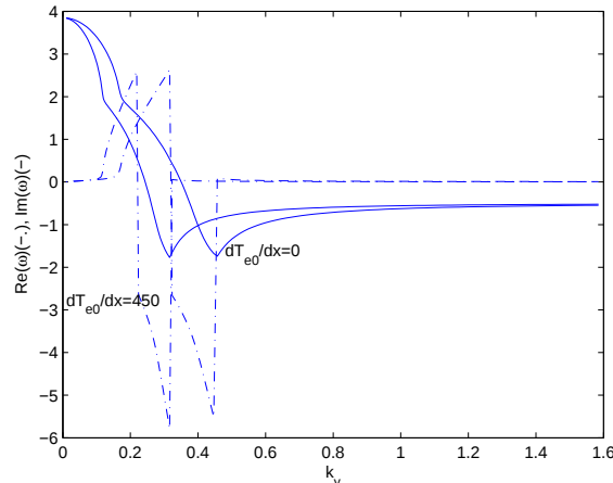
Figure 6. Growth rate (-) and corresponding real part (—) of the most unstable solution of (9) for the following non-dimensional parameters: \tilde{n}_{n0} = 20 , \tilde{v}_{ix0} = -5 , \tilde{v}_{nx0} = -5 , \tilde{\xi}_{i0} = 0.5 , \tilde{\xi}_{e0} = 0 and \tilde{T}_{e0} = 450 . Parametric variation of \tilde{k}_y and d\tilde{T}_{e0}/dx
