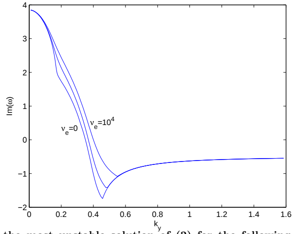
Figure 2. Growth rate of the most unstable solution of (2) for the following non-dimensional parameters: \tilde{n}_{n0} = 20 , \tilde{v}_{ix0} = -5 , \tilde{v}_{nx0} = -5 , \tilde{\xi}_{i0} = 0.5 and \tilde{T}_{e0} = 450 . Parametric variation of k_y and \tilde{\xi}_{e0}
