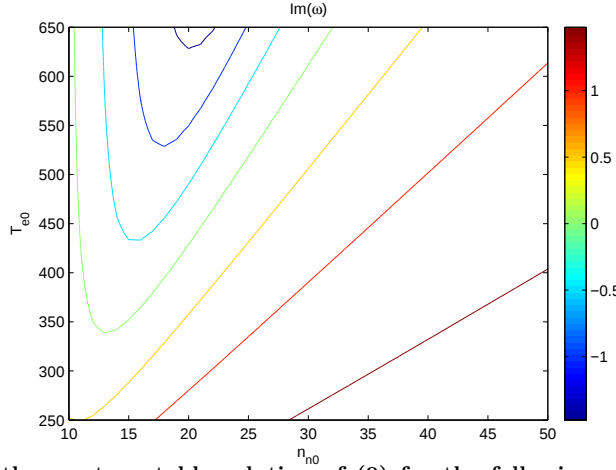
Figure 7. Growth rate of the most unstable solution of (9) for the following non-dimensional parameters: k_y = 0.25 , \tilde{v}_{ix0} = -5 , \tilde{v}_{nx0} = -5 , \xi_{i0} = 0.5 and \xi_{e0} = 0 . Parametric variation of \tilde{n}_{n0} and \tilde{T}_{e0} = d\tilde{T}_{e0}/d\tilde{x}
