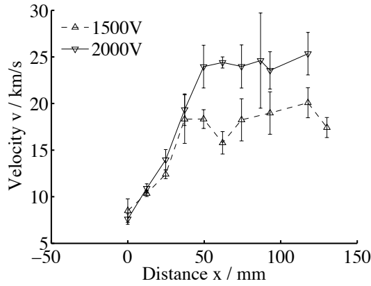
(a) Velocity distribution along the electrodes for 2000 V and 1500 V.
