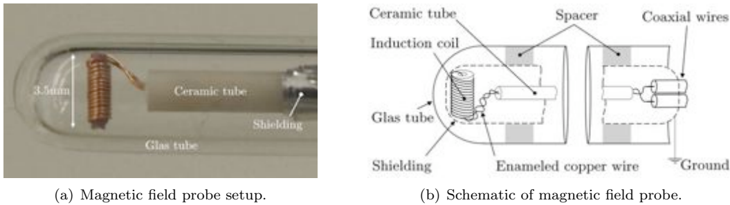
Figure 7. Magnetic field probe, picture and and schematic.
