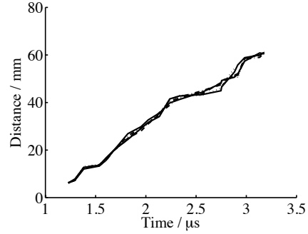
(b) Plasma sheet progression along electrodes from high speed camera.
