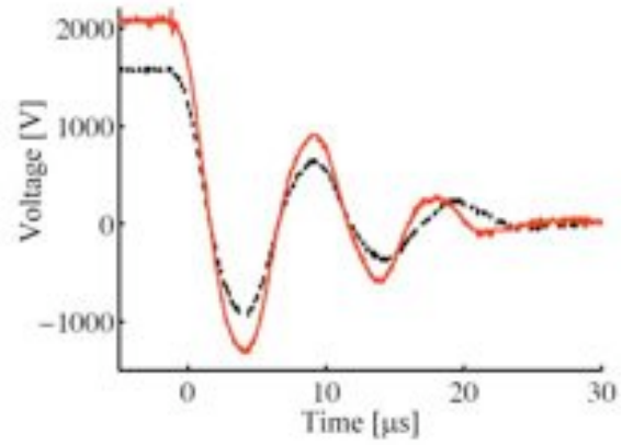
(b) Voltage distribution for 2000 V and 1500 V.
