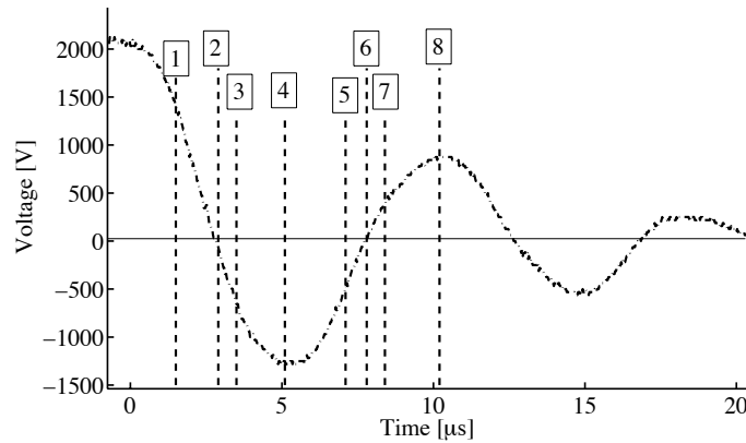
Figure 10. Voltage distribution during discharge. Numbers correlate with pictures in Figure 9.
