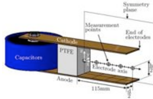
Figure 3. Measurement points along the thruster's axis for Time-of-Flight and Magnetic Field Probe.
