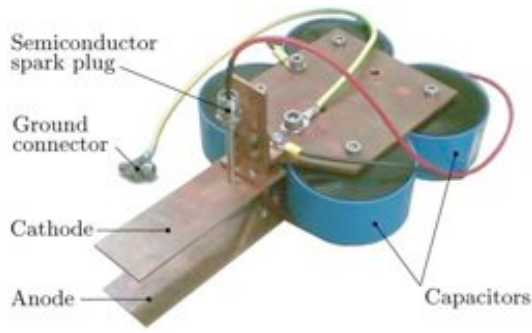
Figure 2. Engineering Model SIMP-LEX.
