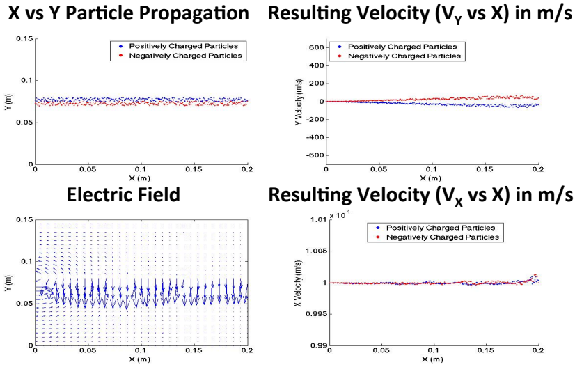
Figure 14. Beam Propagation and Diagnostics with a Beam Width of 0.5 cm
