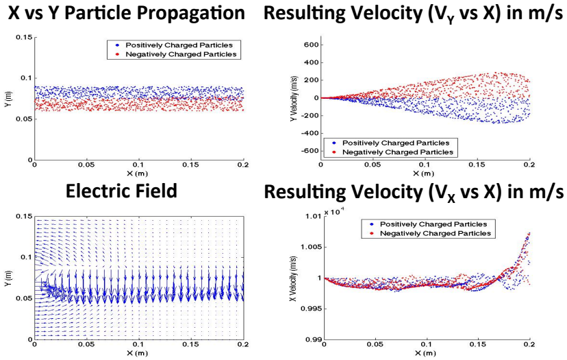
Figure 13. Beam Propagation and Diagnostics with a Beam Width of 1.5 cm
