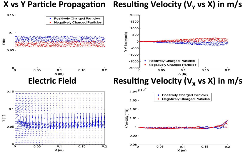
Figure 15. Beam Propagation and Diagnostics with a Current Density of 1 \text{ A/m}^2
