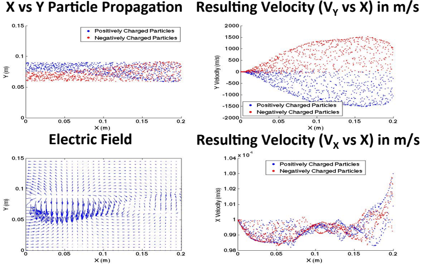
Figure 16. Beam Propagation and Diagnostics with a Current Density of 10 \text{ A/m}^2
