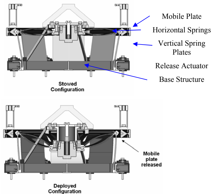
Figure 6. HDRM in stowed and deployed configuration (Principle Drawing)
