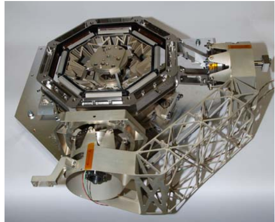
Figure 4. Pointing Arm attached to the HDRM
