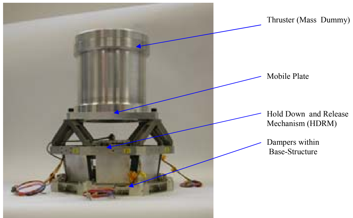
Figure 2. TPM Structure (Breadboard Model)
