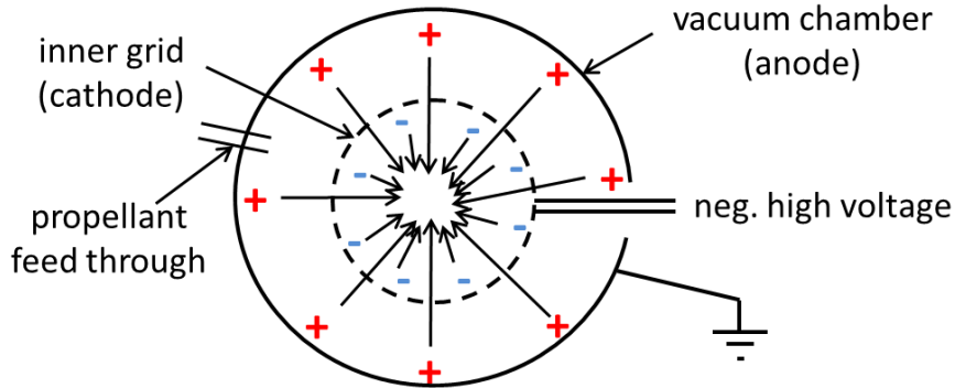
Figure 1. Schematic of a so-called Farnsworth-Hirsch Fusion Reactor.
