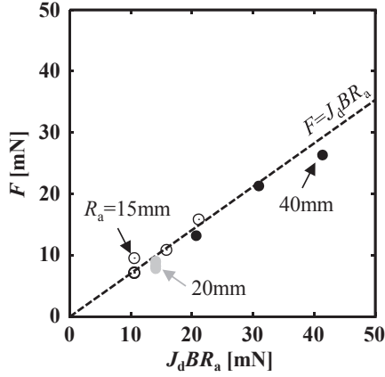
Figure 30. Thrust performance of coaxial AF-MPDT.
