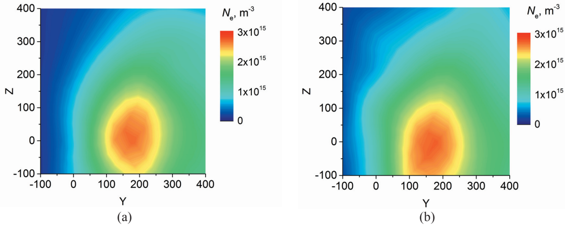
Figure 43. Plasma density at two vacuum conditions. Mass flow rate of 1.36 mg/s, discharge voltage of 250 V.
