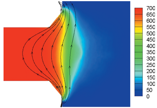
Figure 5. Preliminary simulation result of a 2 kW-class magnetic layer type Hall thruster. Acceleration voltage of 700V was applied to the anode and the displayed plasma potential distribution is time-averaged. The black stream traces denotes the lines of magnetic force. 8
