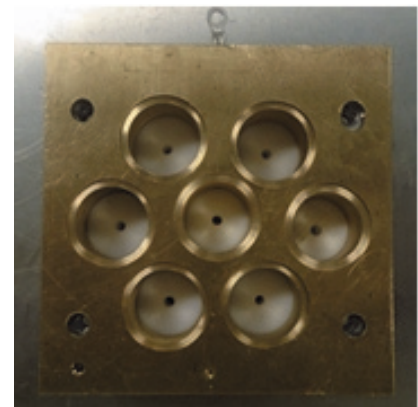
Figure 40. Multi-discharge-room type electrothermal PPT.
