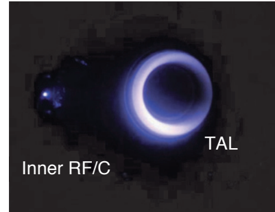
Figure 23. Coupling Phenomena at Inner RF/C Ignition Phase with TAL.
