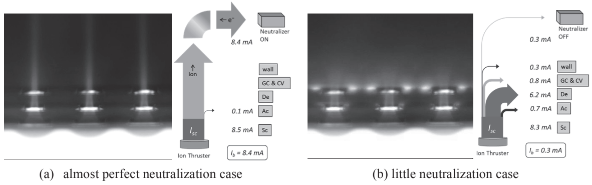
Figure 27. Neutralization phenomena (with visualized ion thruster, 3 grid system)
