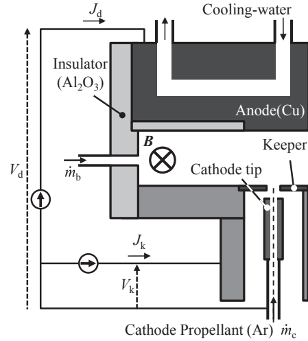
Figure 29. Schematic of rectangular AF-MPDT.
