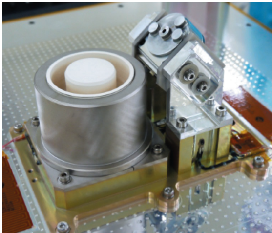
Figure 3. Microwave discharge neutralizer combined with 300W Hall effect thruster for DubaiSat-2.
