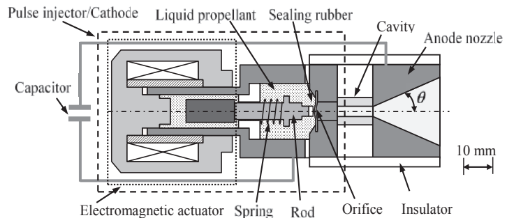
Figure 44. A Liquid Propellant Pulsed Plasma Thruster, Co-axial Electrode Type Thruster with an Anode-Nozzle Area Ratio of 30.
