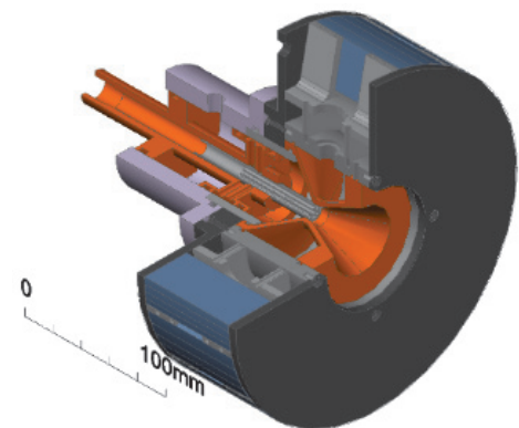
Figure 38. Steady-state water-cooled MPD thruster (3-D Model).
