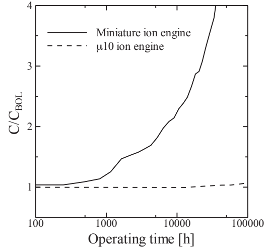
Figure 25. Comparison of change in grid conductance ratio.
