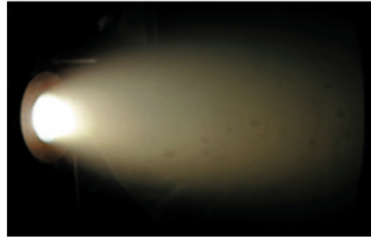
Figure 39. Plasma plume with HAN decomposed gas.
