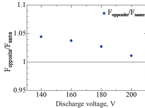
Figure 37. Ratio of thrust for two combinations of magnetic field directions.
