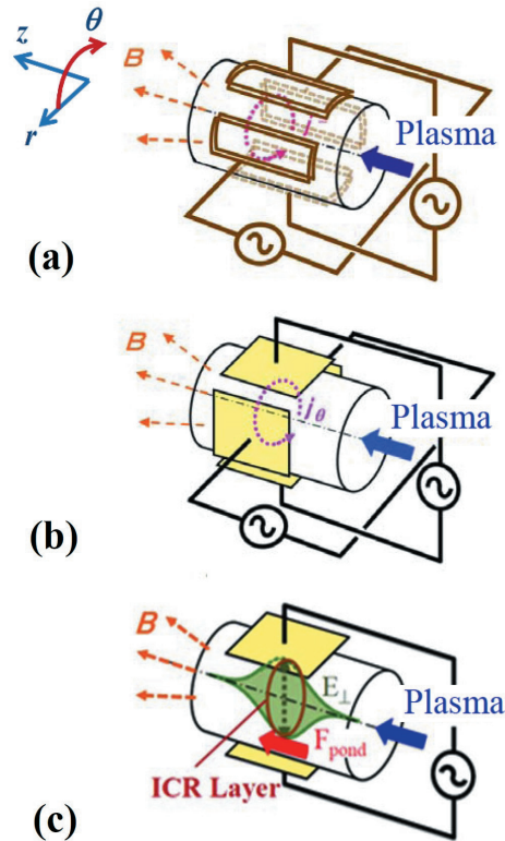
Figure 12. Proposed acceleration schemes: (a) Rotating Magnetic Field (RMF), (b) Rotating Electric Field (REF), and (c) ion cyclotron resonance (ICR) acceleration with a ponderomotive force acceleration (PA).
