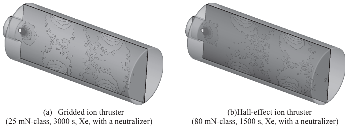
Figure 26. Pressure distribution within a vacuum chamber (2 m in diameter, 5 m in length, 4 pumps)
