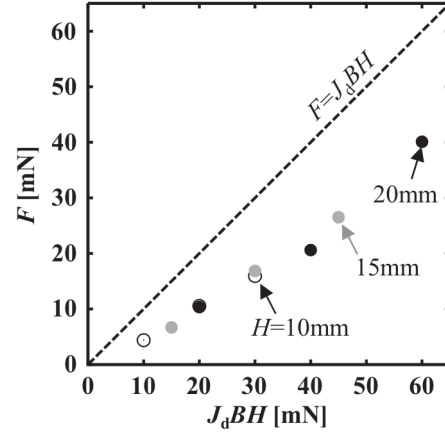
Figure 31. Thrust performance of rectangular AF-MPDT.
