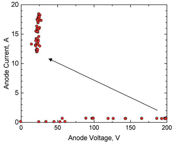
Figure 20. Anode Current with Inner Coil-type RF Plasma Cathode at 200 W RF Power and 2.0 mg/s Xe Mass Flow.
