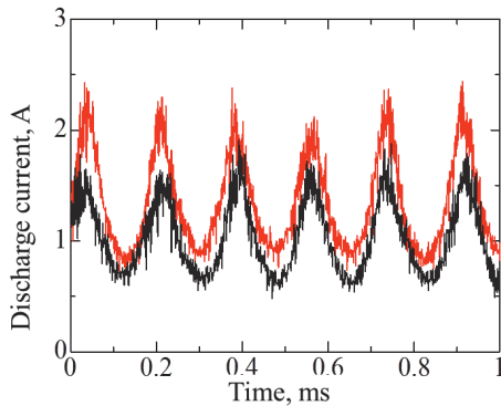
Figure 36. Discharge current profiles for opposite directions of the magnetic fields at 180 V.
