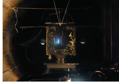
Figure 10. Firing of the ion thruster on the flight model PROCYON.
