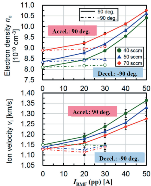
Figure 16. Electron density and argon ion velocity, changing the RMF coil current, gas flow rate, and the phase between two sets of RMF coils.
