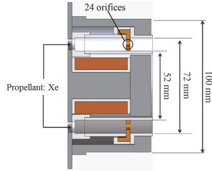
Figure 35. Cross-sectional view of GMK-I.
