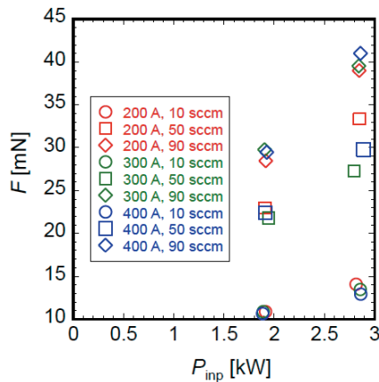
Figure 15. Xenon plasma thrust as a function of rf power, changing the magnetic field coil current and gas flow rate.
