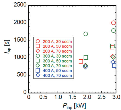
Figure 14. Specific impulse (argon plasma) as a function of rf power, changing the magnetic field coil current and gas flow rate.
