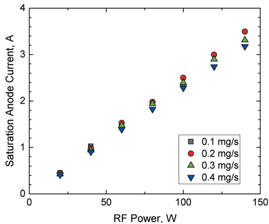
Figure 19. Anode Current from Outer Coil-type RF Plasma Cathode as a function of RF Power.
