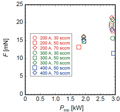
Figure 13. Argon plasma thrust as a function of rf power, changing the magnetic field coil current and gas flow rate.
