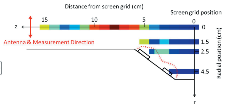
Figure 2. Microwave electric field measurement using an optical fiber with electro-optical device in the microwave discharge plasma source.
