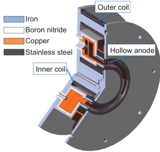
Figure 7. UT-58 thruster with anode layer.
