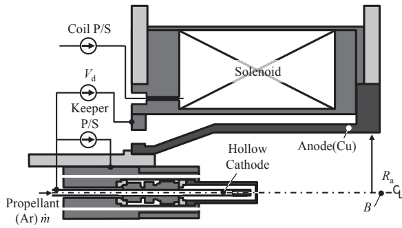
Figure 28. Schematic of coaxial AF-MPDT.
