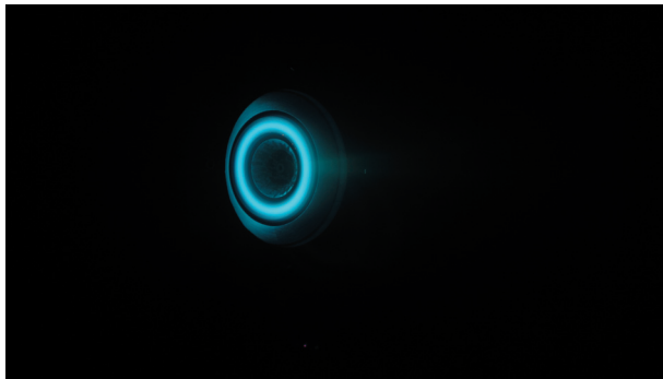
Figure 42. Photo of RAIJIN94. Mass flow rate of 9.8 mg/s, discharge voltage of 300 V.
