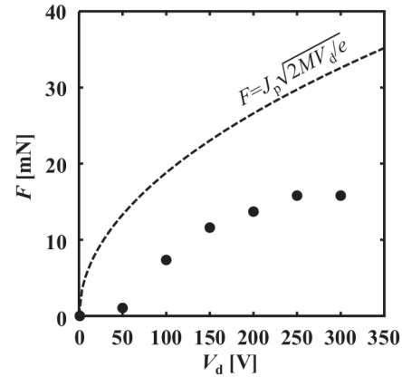
Figure 33. Thrust vs. applied voltage.
