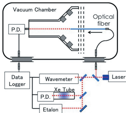
Figure 1. Laser absorption spectroscopy using an optical fiber in the microwave discharge plasma source.
