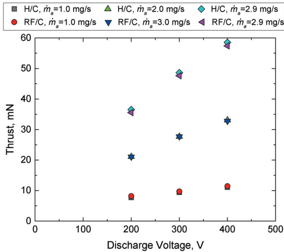
Figure 22. Thrust Comparison between H/C and Outer Coil-type RF/C.
