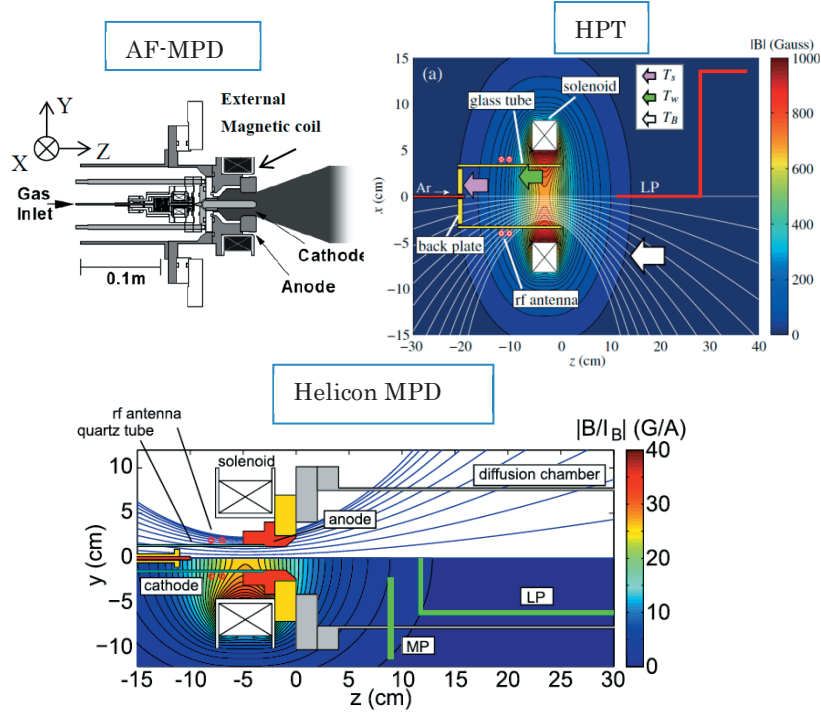
Figure 6. Schematic diagrams of various magnetic nozzle plasma thrusters at Tohoku University.
