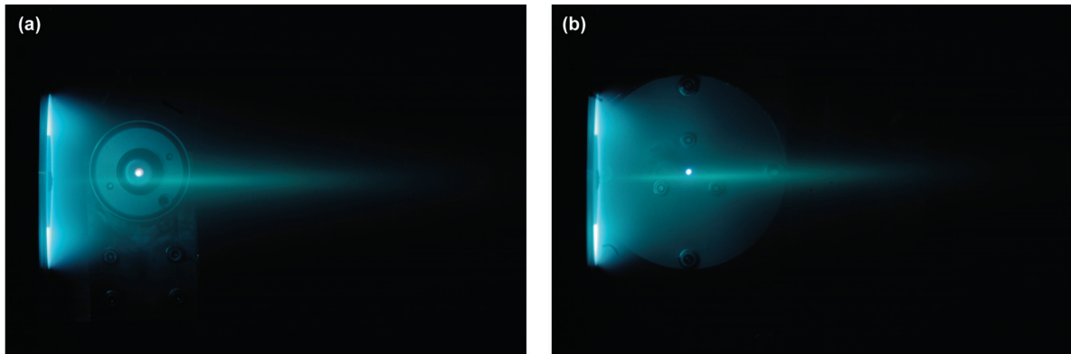
Figure 21. Photos of Thruster Firing at 300V Discharge Voltage, 2.9 mg/s Anode Mass Flow Rate and 0.3 mg/s with (a) Hollow Cathode and (b) Outer Coil-type RF Plasma Cathode.
