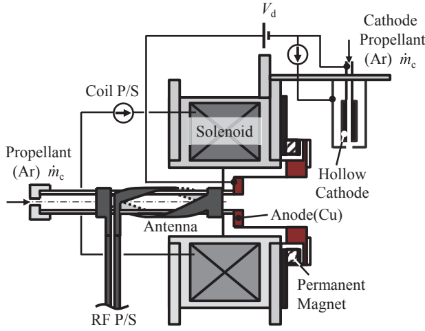
Figure 32. Helicon plasma electrostatic thruster.
