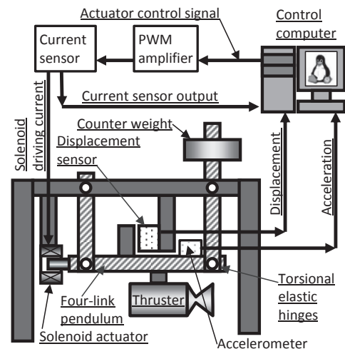
Figure 45. Prototyped thrust stand using null balance method and acceleration compensation.
