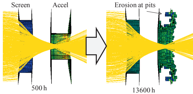
Figure 24. Ion beam trajectories and grid surfaces.
