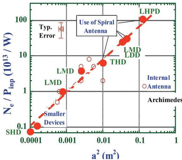
Figure 11. N_e/P_{\text{inp}} vs a^2 for different helicon sources. Here, red closed circles show the data taken by our group.
