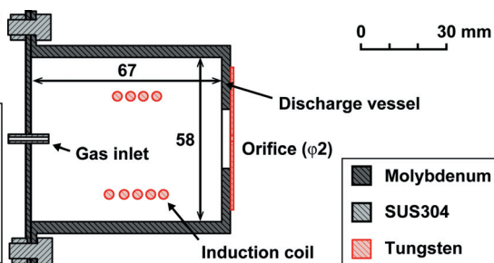
Figure 18. Cross Section of Inner Coil-type RF Plasma Cathode.
