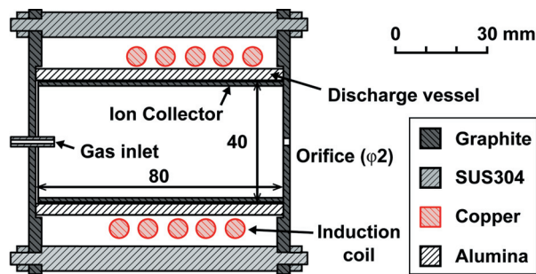
Figure 17. Cross Section of Outer Coil-type RF Plasma Cathode.
