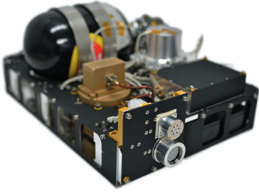
Figure 9. Flight model of the MIPS.
