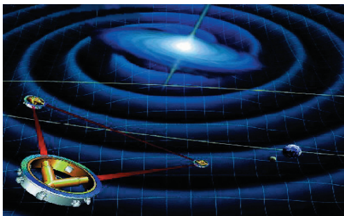
Figure 3: Principle of the LISA mission
