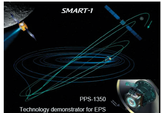
Figure 4: SMART-1 mission
