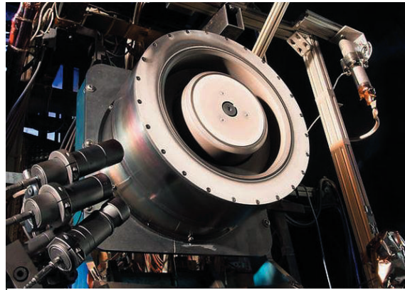
Figure 8. Photograph of the HERMeS thruster used in this investigation. Optical probes are shown to the lower left.
