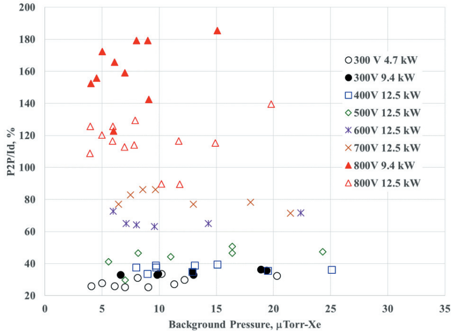
Figure 16. TDU1 P2P/Ia percent variation as a function of background pressure for various thruster operating conditions.
