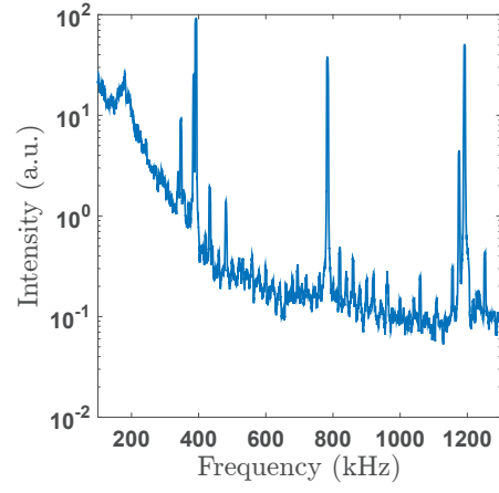
(b) Cathode power spectrum. B = B^*
