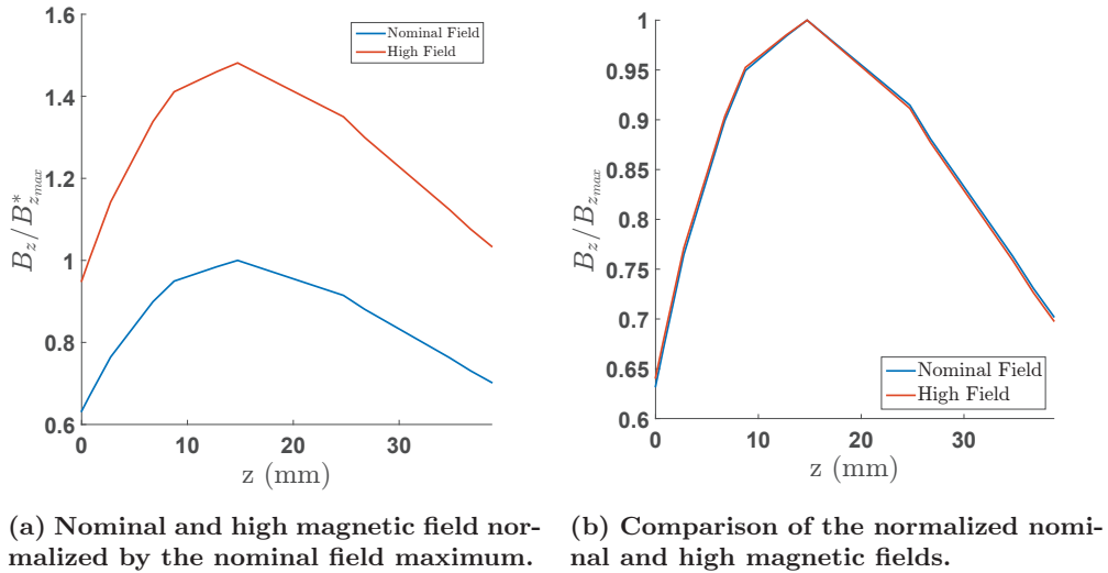
Figure 6: Comparison of the high and low magnetic field conditions, highlighting that the topology has not changed between the conditions.
