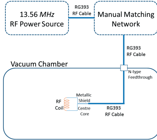
Figure 3. Radio frequency power setup of the RF plasma cathode experiments
