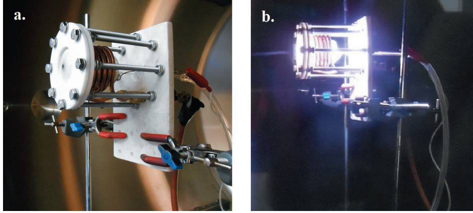
Figure 4. Pictures of the RF cathode test setup a) inside the vacuum chamber and b) during its operation
