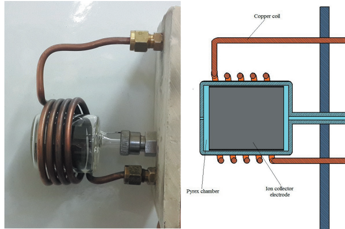
Figure 1. 2D drawing and the picture of the manufactured prototype RF plasma cathode
