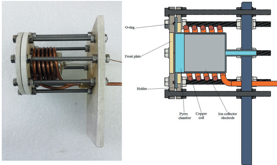
Figure 2. 2D drawing and picture of the new prototype RF plasma cathode
