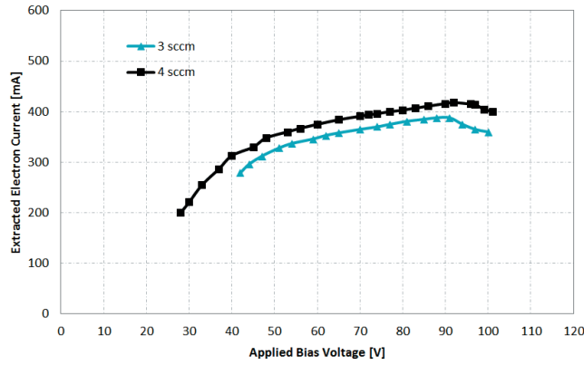
Figure 6. I-V characteristics of the RF plasma cathode for 3 sccm and 4 sccm argon gas flow rates at 40 W RF power
