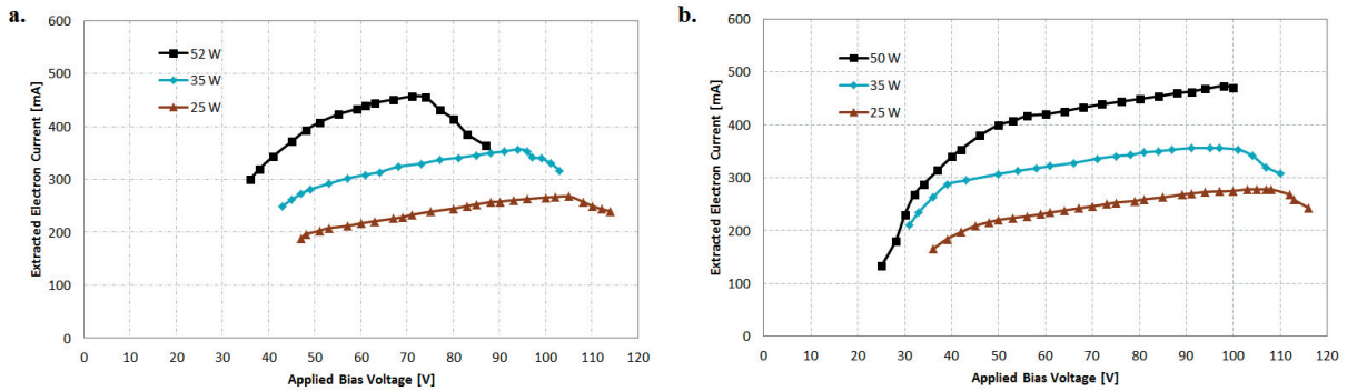
Figure 5. I-V characteristics of the RF plasma cathode for a) 3sccm and b) 4sccm of argon gas flow rates at various RF power values
