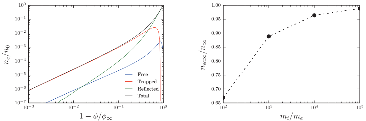
Figure 8. Contribution to the total density of each electron population along the expansion (left) and the ratio between the final confined electron density n_{e\infty} and the final total density n_\infty for different mass ratio profiles (right).
