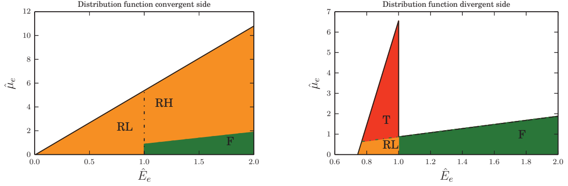
Figure 4. Electron distribution function for the profile m_i/m_e = 10000 and T_{i0}/T_{e0} = 1.0 at two different local positions, \frac{\phi}{\phi_\infty} = 0.05 for the convergent region and \frac{\phi}{\phi_\infty} = 0.72 for the divergent region. “RH” represents the high energy reflected electrons, “RL” stands for the low energy reflected electrons, “F” corresponds to the free electron population and finally “T” represents the trapped electrons (only existing in the divergent region of the expansion)
