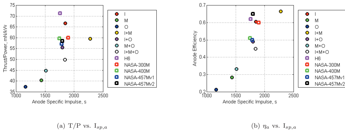
Figure 10. Performance metrics of the X3 compared to other state-of-the-art Hall thrusters at similarly low current densities.
