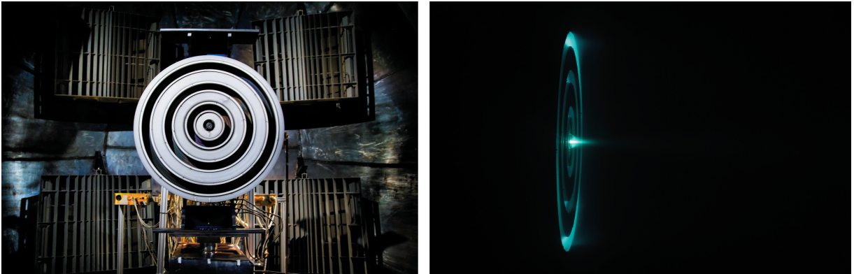
Figure 1. The X3 100-kW class nested Hall thruster mounted for operation inside the Large Vacuum Test Facility at the University of Michigan (left) and firing in three-channel configuration at 30 kW (right).
