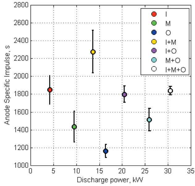
Figure 5. Anode specific impulse versus discharge power across all operating conditions.
