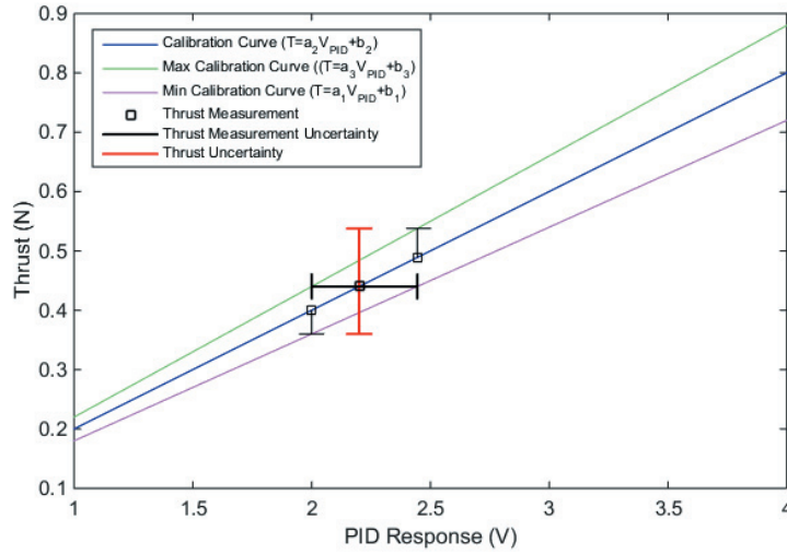
Figure 11. An example plot of the thrust stand calibration curves, a thrust measurement, and the associated uncertainty in the measurement.
