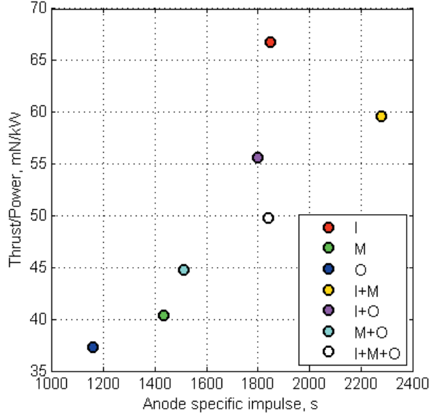
Figure 7. Thrust-to-power ratio versus anode specific impulse.
