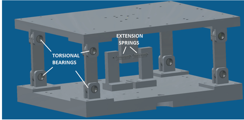
Figure 3. A computer model of the support and spring system used in the X3 thrust stand, with the torsional bearings and extension springs highlighted.
