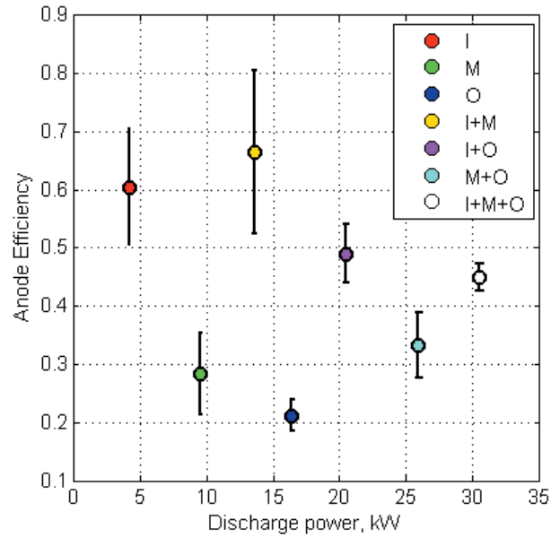
Figure 6. Anode efficiency versus discharge power across all operating conditions.
