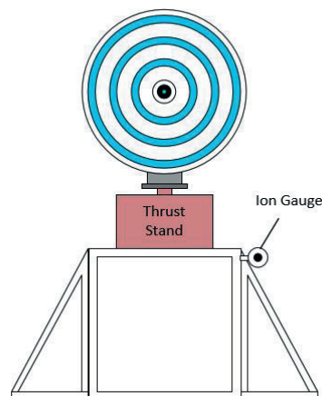
Figure 2. Schematic of ion gauge location relative to thruster.
