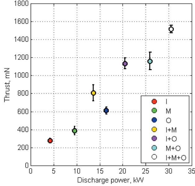
Figure 4. Thrust versus power across all operating conditions.
