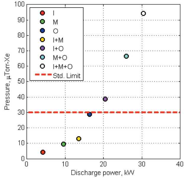
Figure 8. The backpressure at each operating condition as compared to the maximum backpressure for Hall thruster performance measurements as stated in the industry standards guide. 13
