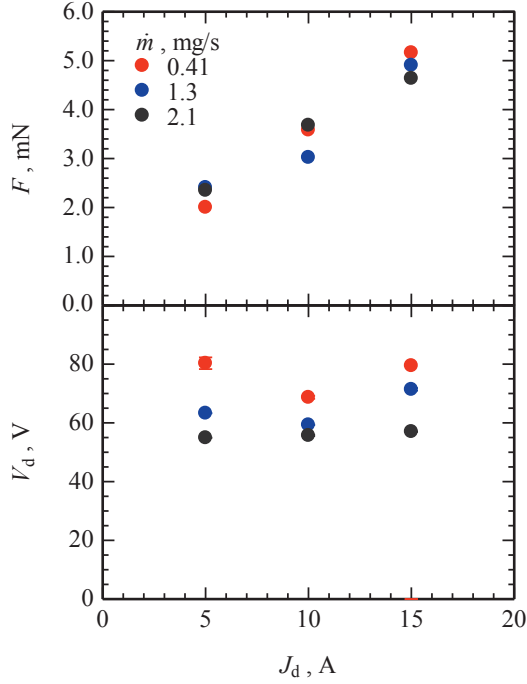
Figure 7 F and V_d of cylindrical type Af-MPD thruster as a function of J_d . \dot{m}=0.41\text{-}2.1\text{mg/s} , B=265\text{ mT} , R_a=15\text{ mm} , z_{\text{cathode tip}}=0\text{mm} .
