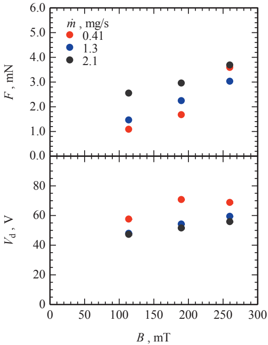
Figure 9 F and V_d of cylindrical type Af-MPD thruster as a function of B . \dot{m}=0.41\text{-}2.1\text{mg/s} , J_d=5\text{-}15\text{ A} , R_a=15\text{ mm} , z_{\text{cathode tip}}=0\text{mm} .
