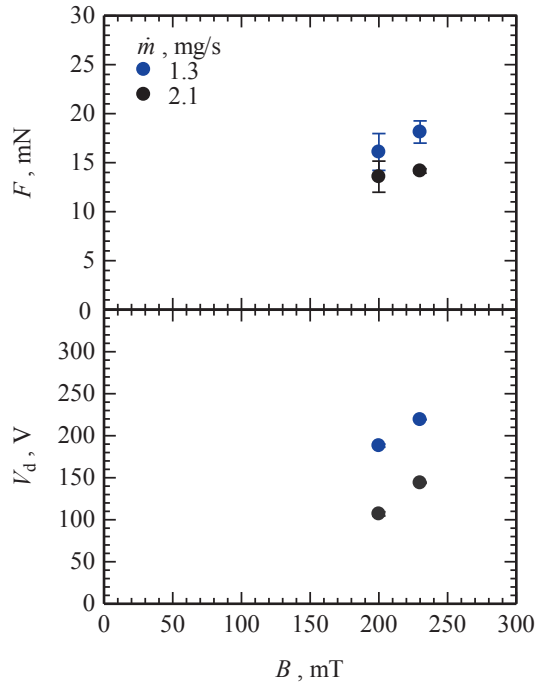
Figure 10 F and V_d of rectangular type Af-MPD thruster as a function of B . \dot{m}=0.41\text{-}2.1\text{mg/s} , J_d=5\text{-}15\text{ A} , H=10\text{ mm} , z_{\text{cathode tip}}=19\text{mm} .
