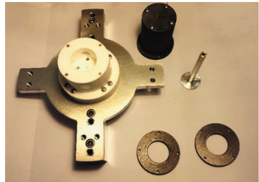
Figure 4: Heaterless hollow cathode disassembled
