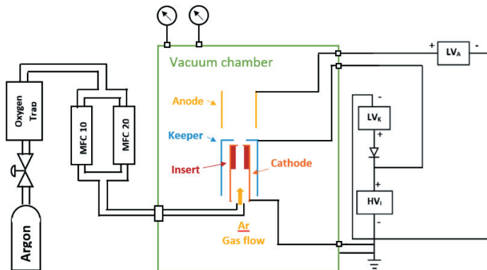
Figure 2: Schematic of the electrical and propellant setup
