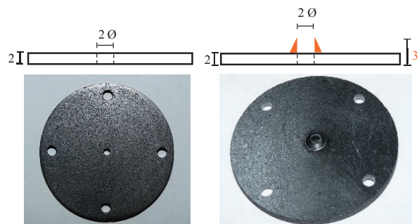
Figure 7: original 2 mm keeper (left), sharp keeper orifice with side view schematic above, dimensions in mm
