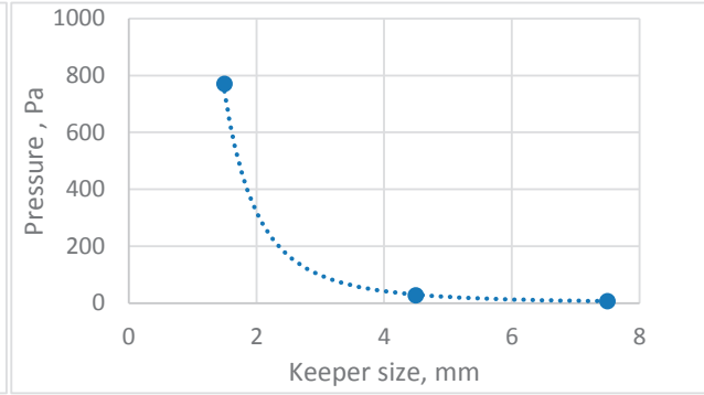
Figure 15: Pressure variation with keeper orifice size, 20 sccm flow rate, 3 mm gap, 1.5 mm cathode orifice
