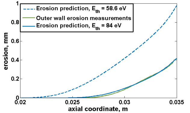
Figure 9. Erosion prediction with different energy thresholds against erosion measurements after 33 h of firing
