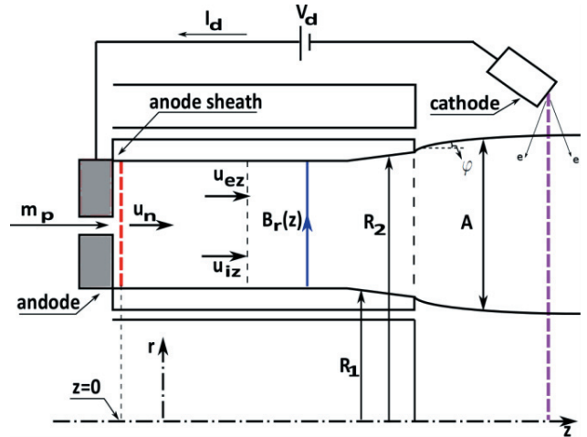
Figure 1. Hall thruster geometrical scheme
