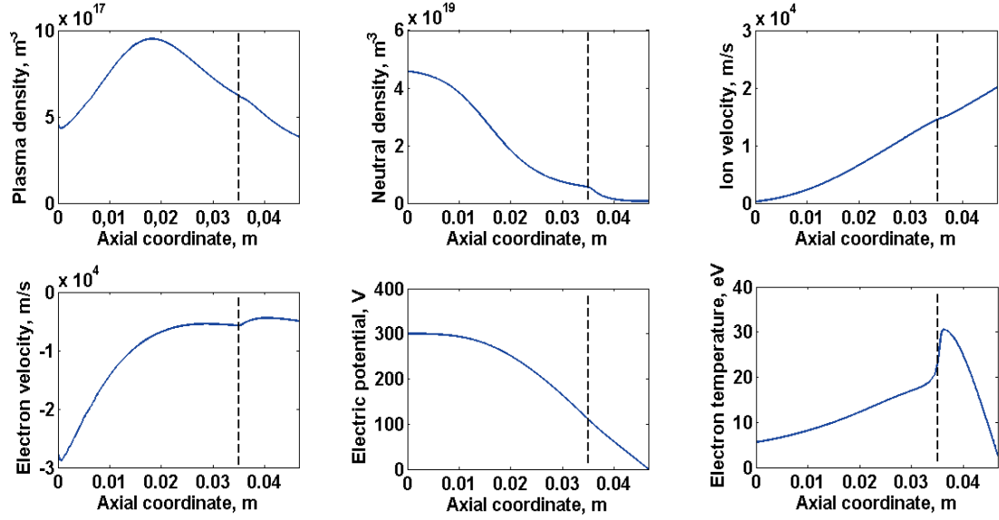
Figure 5. HT5k plasma proprieties, with Kr as propellant. Thruster operating point: V_d = 300 V, \dot{m}_p = 12 \frac{mg}{s} , I_d = 16.8 A, P = 5040 W. The dashed lines indicate the axial location of the channel exit.
