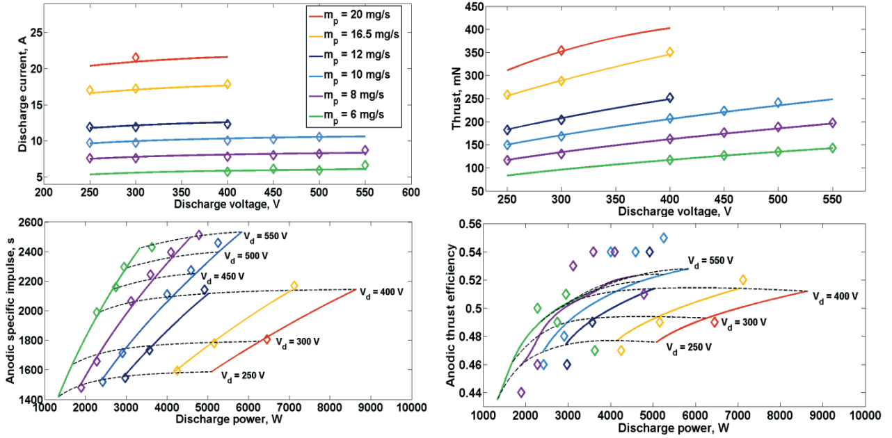
Figure 6. Comparison between predicted performance parameters and experimental data of the HT5k operating with xenon.
