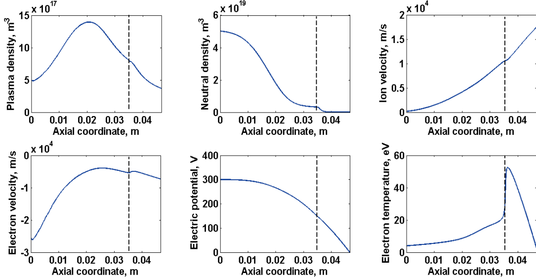
Figure 4. HT5k plasma proprieties, with Xe as propellant. High thrust nominal operating point: V_d = 300 \text{ V} , \dot{m}_p = 16.5 \frac{\text{mg}}{\text{s}} , I_d = 16.7 \text{ A} , P = 5000 \text{ W} . The dashed lines indicate the axial location of the channel exit.
