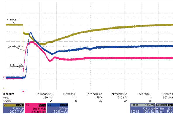
Figure 10 : Thruster start-up
