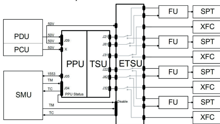
Figure 4. SmallGEO EPTA
