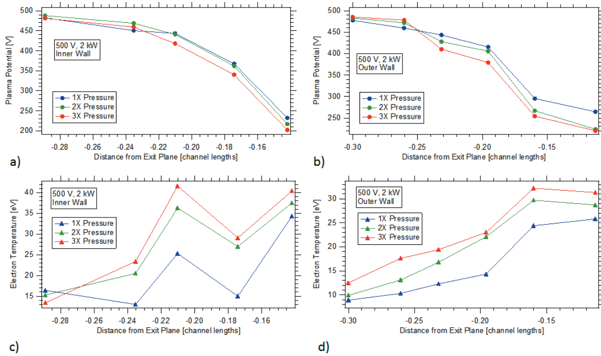
Figure 8. Comparison of measured plasma potentials (with respect to cathode potential) and electron temperatures along the channel walls at 500 V, 2 kW for various facility backpressures.
