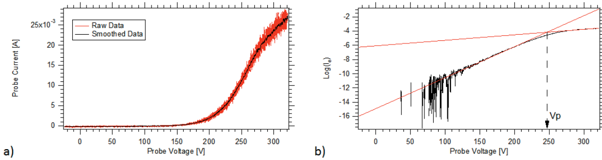
Figure 4. (a) Example Langmuir probe I-V characteristic, plotted both before and after boxcar averaging was performed. (b) Semi-log plot of corresponding electron current and determination of electron temperature and plasma potential.
