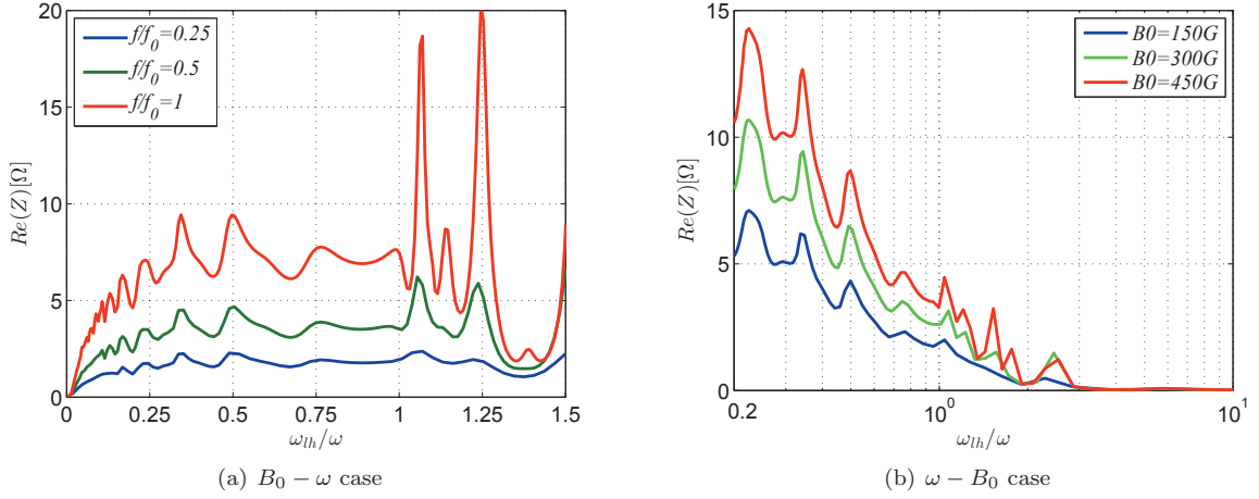
Figure 10. Plasma resistance versus magnetic field and wave frequency. Figure a shows the resistance as a function of magnetic field with different frequency. The nominal frequency f_0 is 13.56\text{MHz} . Figure b shows the resistance as a function of frequency with different magnetic fields.
