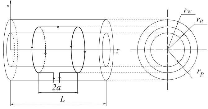
Figure 1. Helicon source model.
