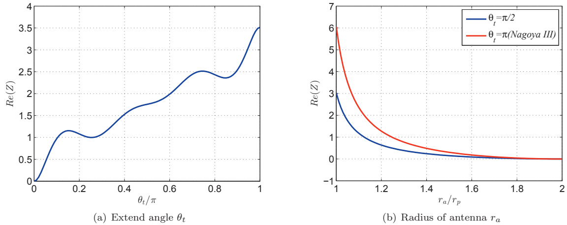
Figure 3. Resistance varying with the extend angle \theta_t and antenna radius r_a for double saddle antenna family.
