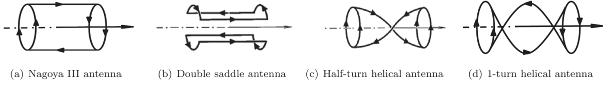
Figure 2. Different types of antennas.
