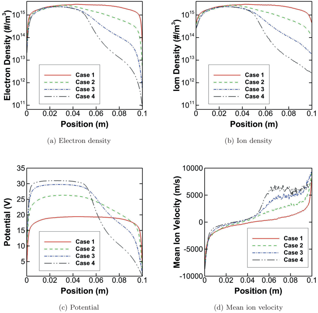
Figure 9: Set 3, full simulations with magnetic field forces and area variation.
