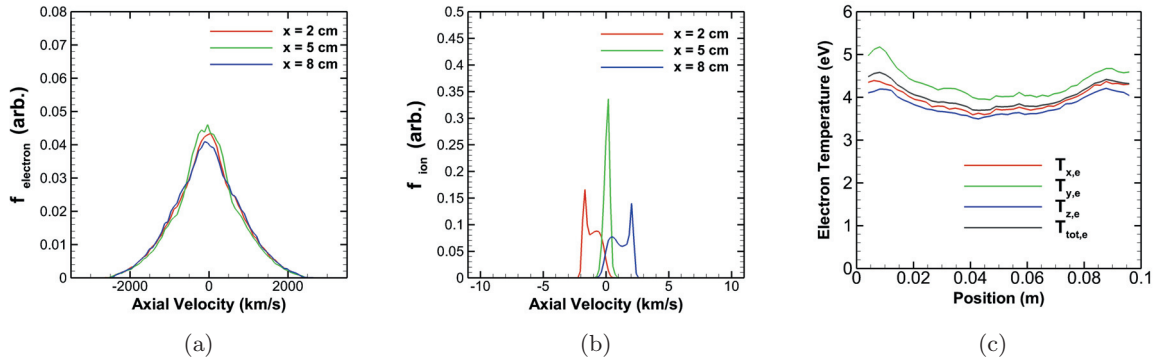
Figure 6: Set 1-4, Case 1 simulation results. (a) Electron axial velocity distribution. (b) Ion axial velocity distribution. (c) Spatial electron temperatures.
