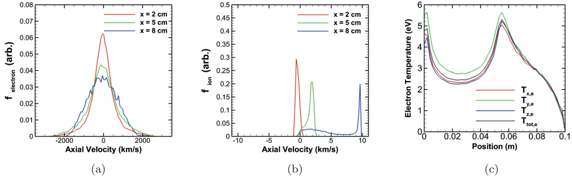
Figure 11: Case 4 results with no ion magnetization, magnetic forces on electrons, and cross-sectional area variation. (a) Electron axial velocity distribution, (b) Ion axial velocity distribution, (c) Spatial electron temperature variation.
