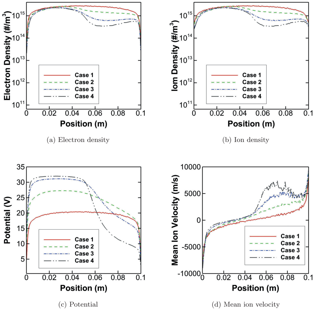
Figure 8: Set 2, magnetic field force simulations.
