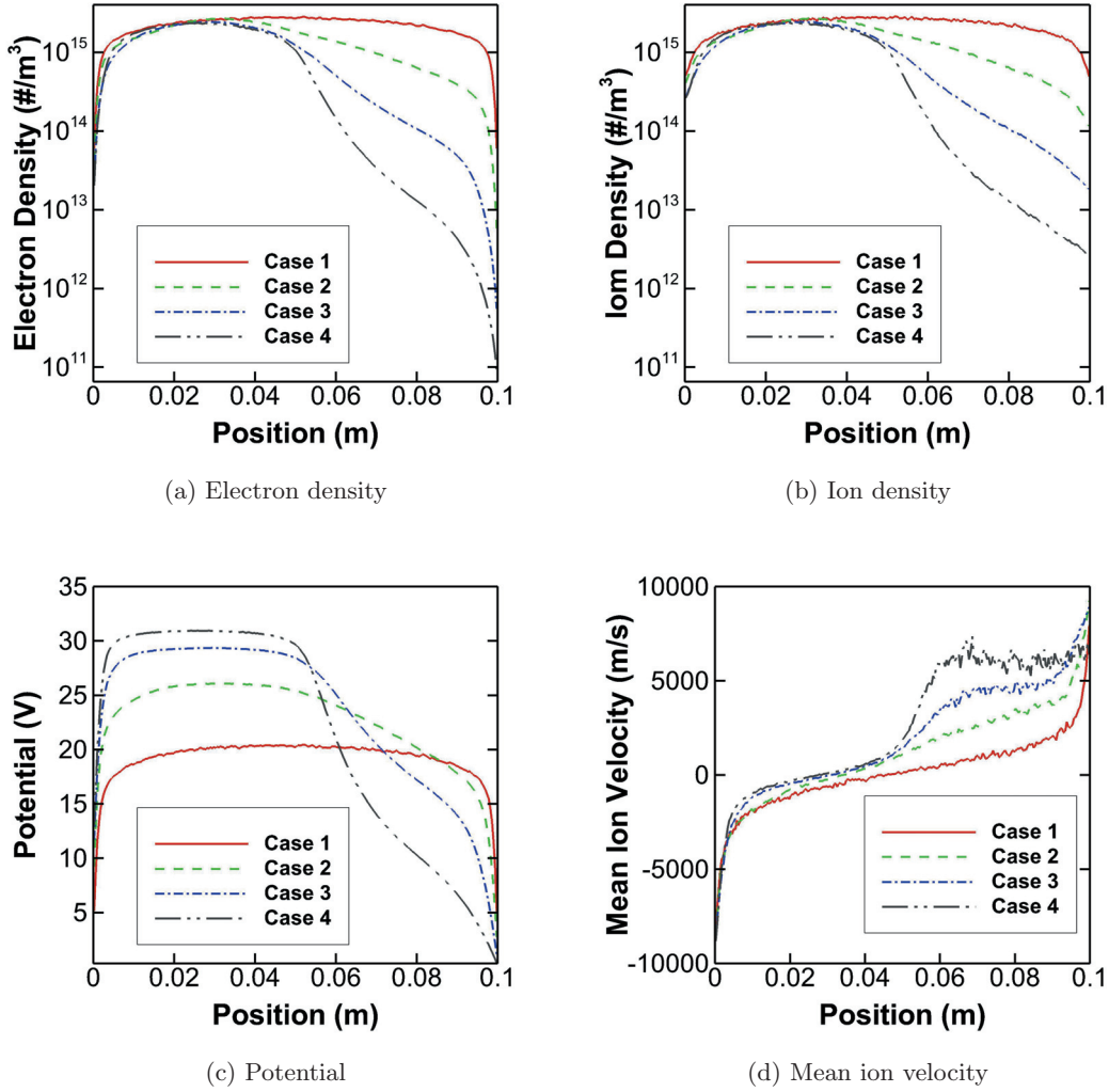
Figure 10: Set 4, full simulations with magnetic field forces only on the electrons and cross-sectional area variation.
