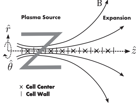
Figure 3: Quasi-1D particle simulation domain resolving the centerline axis as shown by the cells.
