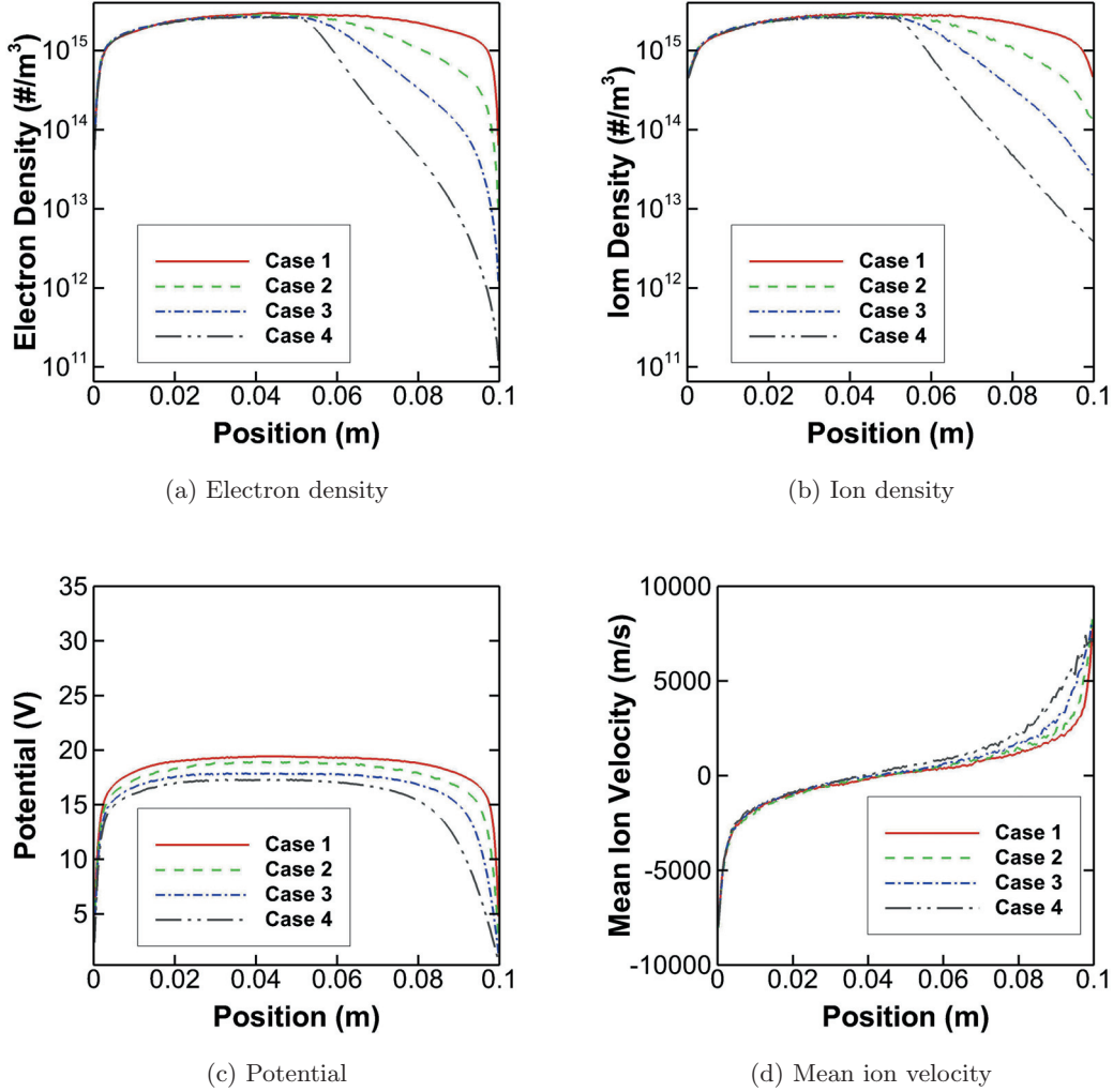
Figure 7: Set 1, density effect simulations.
