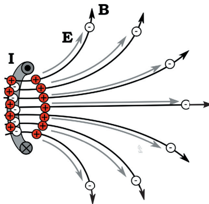
Figure 2: Electric field generated in a magnetic nozzle by electron thermal expansion along a magnetic field.
