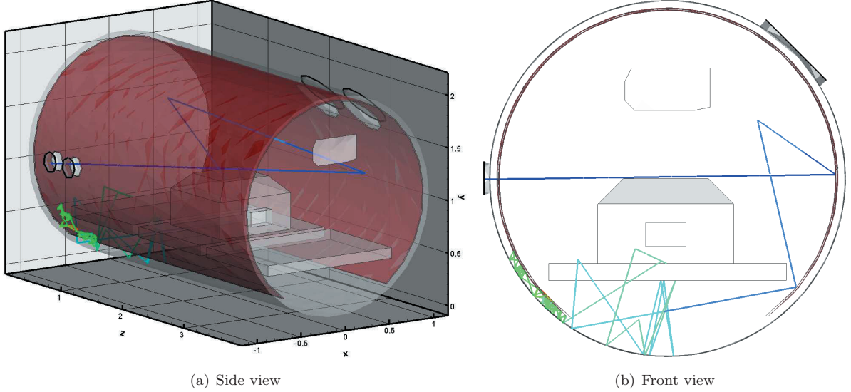
Figure 3. Plot of a single particle trace and also the setup geometry. The particle is injected at a port plate, and after a large number of surface impacts, ends up in the narrow space between the thermal shroud and the chamber wall. The cryopumps, small scavenger plate, platens, and test hardware can also be seen.
