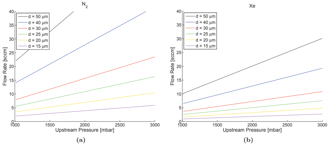
Figure 4: The nominal expected mass flow rate of a) nitrogen and b) xenon through a given COTS orifice size with the range of pressures upstream of the orifice that the pressure regulator can deliver.
