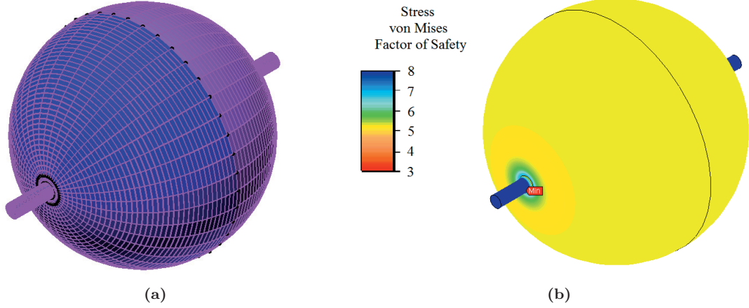
Figure 3: The a) finite element mesh and b) resulting stress factor of safety for the titanium tank with an internal pressure of 100 bar. The red arrow indicates where the minimum factor of safety was encountered.
