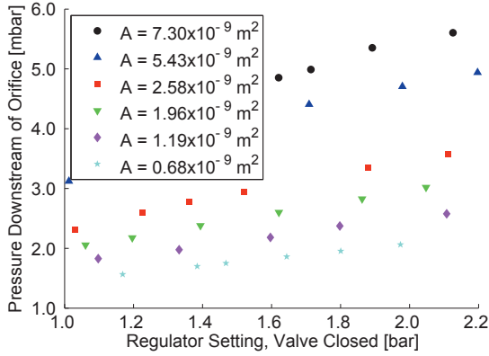
Figure 9: The pressure downstream of the orifice when propellant is flowing through the system compared to the actual regulated pressure setting.
