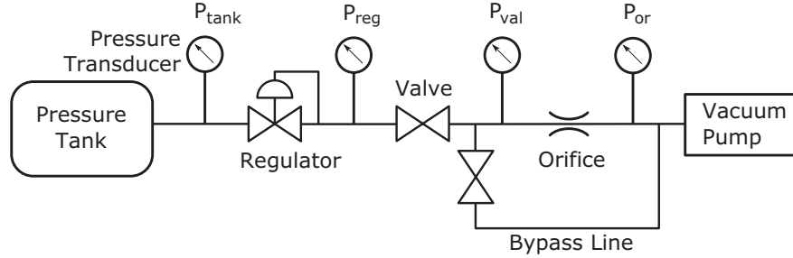
Figure 6: A schematic of the propellant feed system characterization experimental setup.
