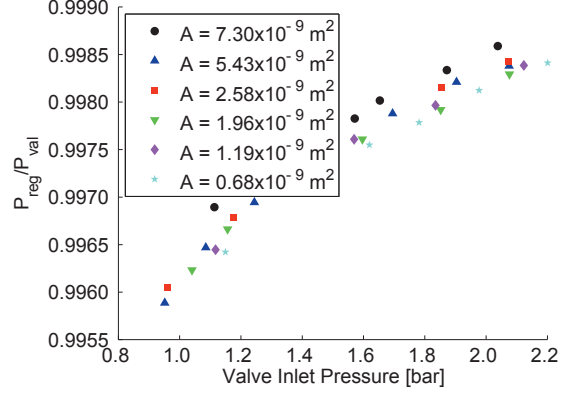
Figure 8: The pressure at the inlet and outlet of the valve. Since the two are equal, within error bars, the effective pressure drop across the valve is negligible.
