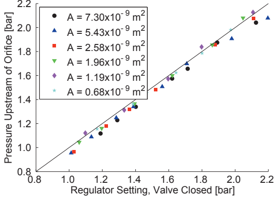
Figure 7: The pressure upstream of the orifice when propellant is flowing through the system compared to the actual regulated pressure setting.
