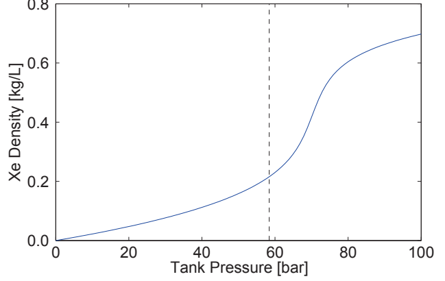
Figure 1: The density of xenon as a function of pressure, as reported by NIST. 19 The dashed line indicates the pressure at which xenon goes supercritical.
