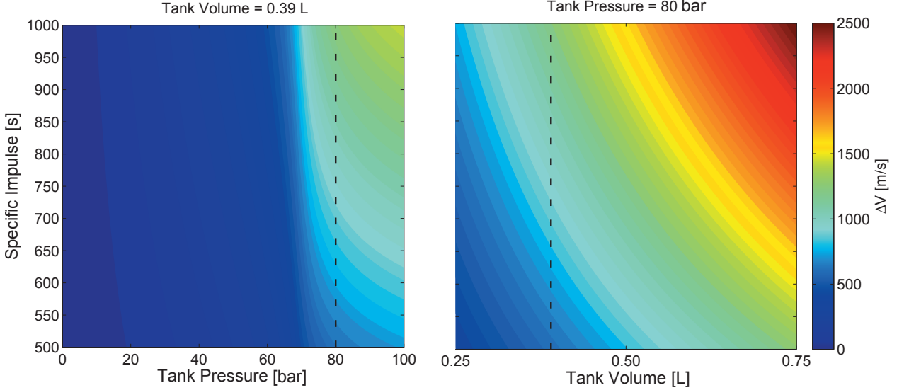
Figure 2: The \Delta V provided to a representative CubeSat as a function of thruster specific impulse and xenon propellant tank pressure (left) and volume (right). The results in the left figure use a tank volume of 0.39 L and in the right figure use a tank pressure of 80 bar.
