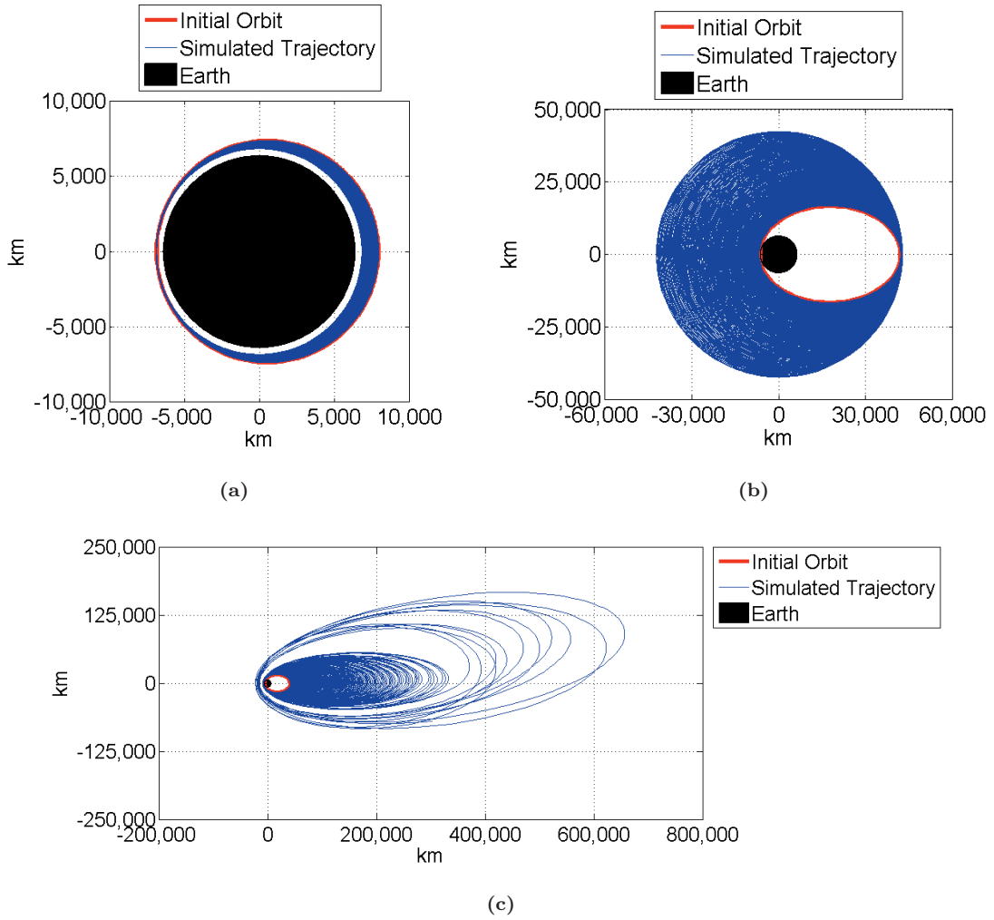
Figure 11: Example spacecraft maneuvers using CAT and a propellant management system similar to the one outlined in this paper. a) An example orbit circularization maneuver. b) An example GTO to GEO insertion maneuver. c) An example Earth escape maneuver with lunar perturbations.
