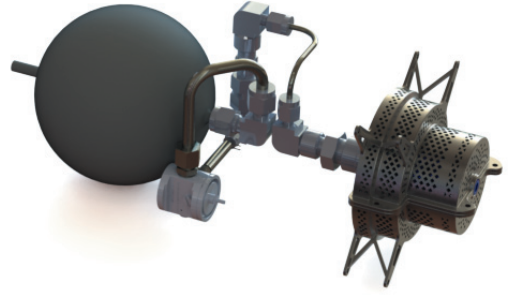
Figure 5: A notional propulsion system layout, using prototype hardware, for integration into a CubeSat bus to check the envelope requirement.
