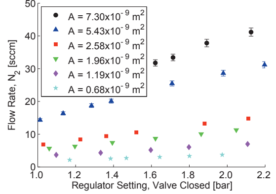
Figure 10: The flow rate of \text{N}_2 when propellant is flowing through the system compared to the actual regulated pressure setting. Data points without error bars have uncertainty ranges smaller than the size of the point.
