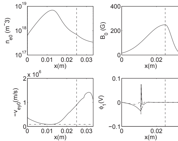
Figure 6. Same as Fig. 1 with background solution B4 and Model 3.
