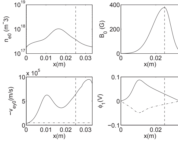
Figure 8. Same as Fig. 1 with background solution D3 and Model 2.
