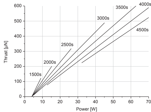
Figure 9 Performanca map of the IFM 350 Nano as measured by direct thrust measurements
