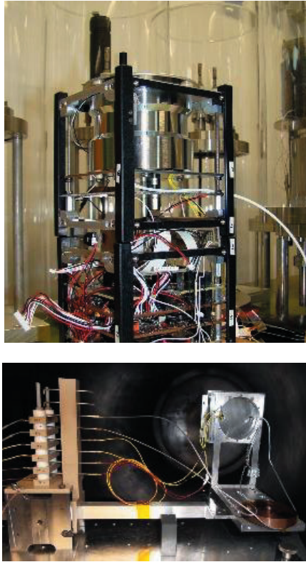
Figure 8 top: IFM 350 Nano thruster integrated in an ISIS Cubesat Structure, bottom: IFM 350 Nano thruster on the FOTEC \mu\text{N} thrust balance
