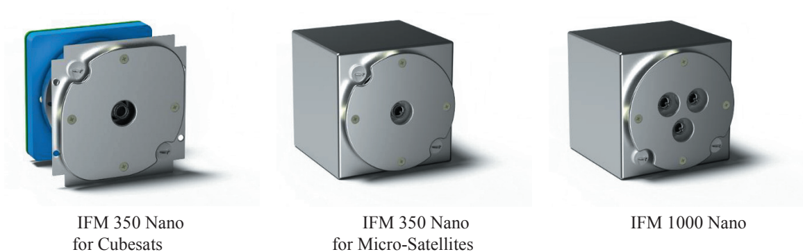
Figure 4 The IFM Nano Thruster Family. The outer dimensions of all modules do not exceed 10x10x10cm.
