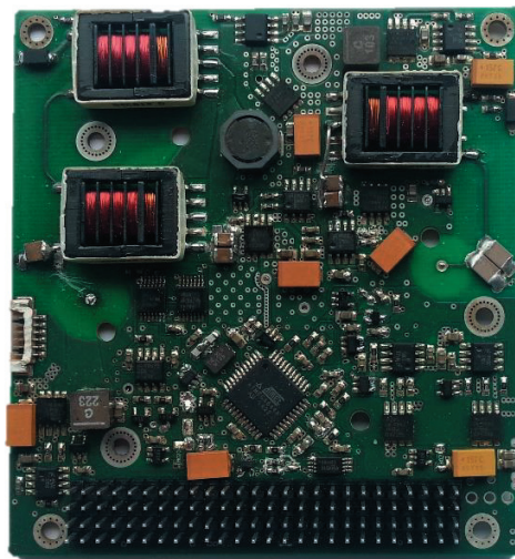
Figure 7 Prototype of FEEP power suitable for standard CubeSat bus.
