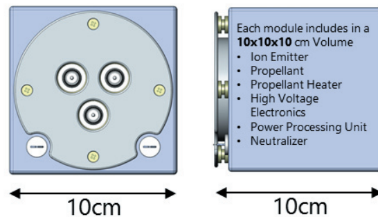
Figure 5 Highly integrated design concept of the IFM Nano thruster family
