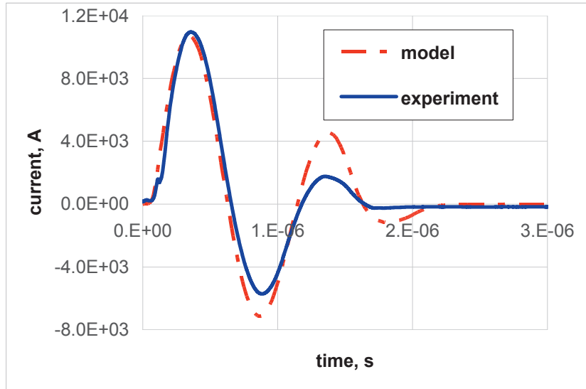
Figure 2. Comparison of predicted and measured current for PPT chamber given in Fig.1.
