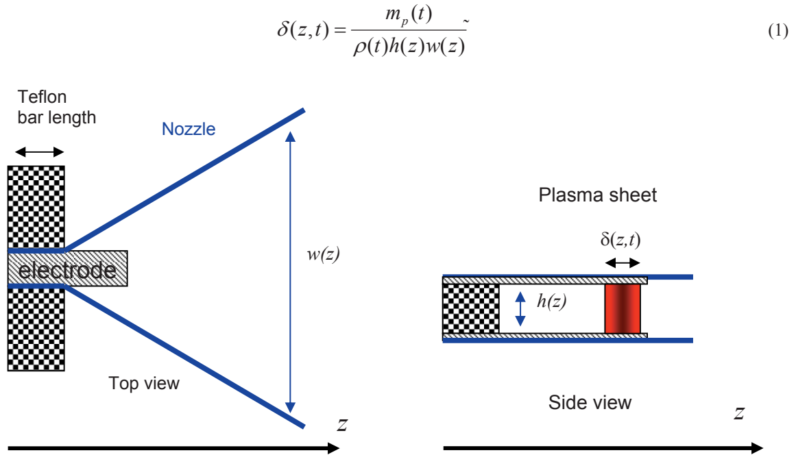
Figure 1. Model Geometry of PPT chamber.
