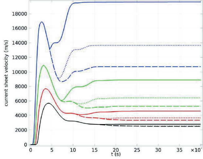
Figure 5. Predicted velocity of the current sheet: color code for distance between electrodes (blue – 8mm, green – 10mm, red – 12mm, black – 14mm), line style for different length of Teflon bars: solid – 5mm, dotted – 7mm, dashed – 9mm.
