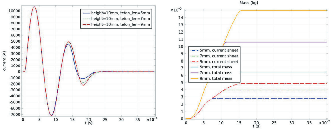
Figure 6. Predicted effect of the propellant bars length (a) current waveforms; (b) total ablated mass and ionized fraction.
