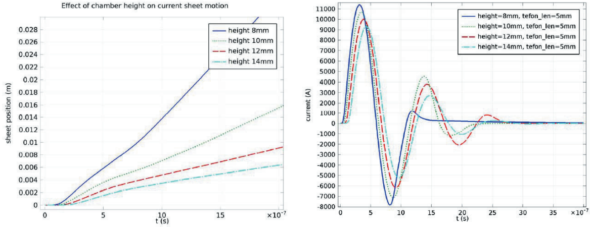
Figure 3. Predicted effect of the distance between electrodes on motion of the current sheet and the current. (a) sheet position (compare with Teflon bars length 0.005m); (b) current waveform
