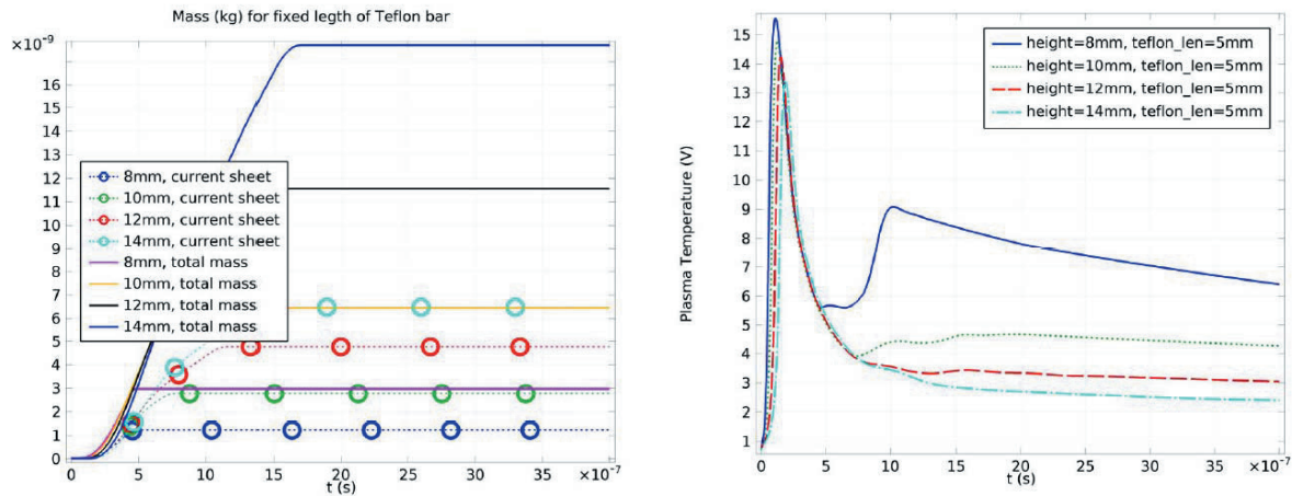
Figure 4. Predicted effect of the distance between electrodes on (a) total ablated mass and ionized fraction; (b) plasma temperature in eV.
