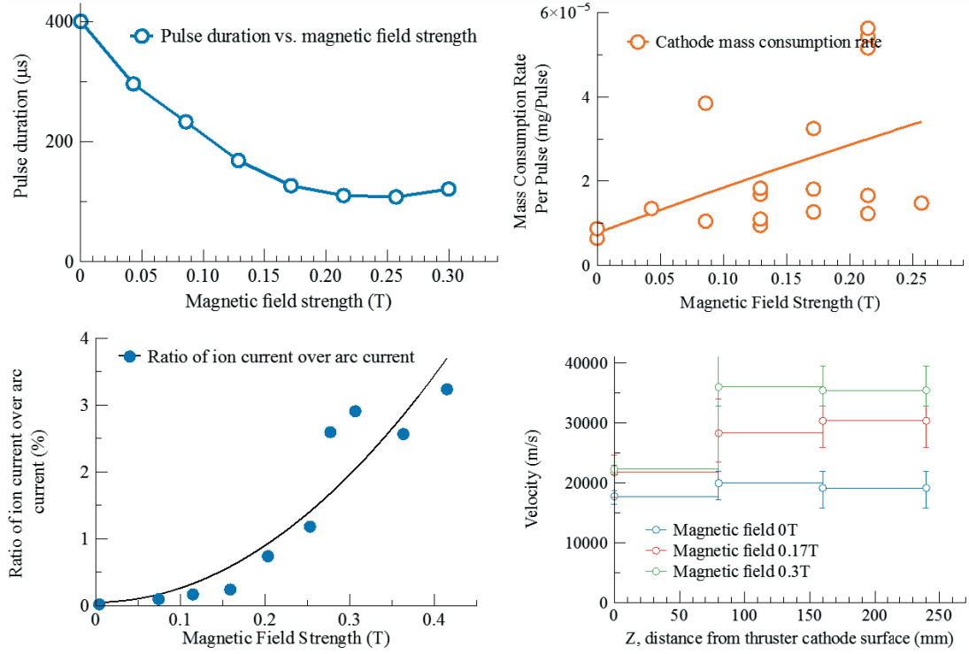
Figure 2. Summary of thruster operating parameters. Figure from 1.
