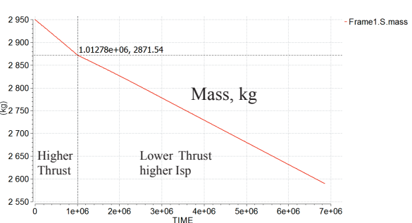
Figure 6. Total satellite mass evolution
