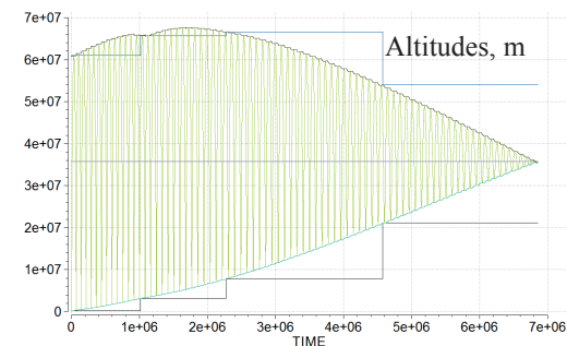
Figure 5. Apogee, Perigee altitudes and Optimiser data
