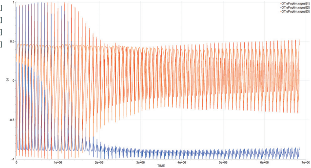
Figure 8. Thrust orientation evolution wrt ECI
