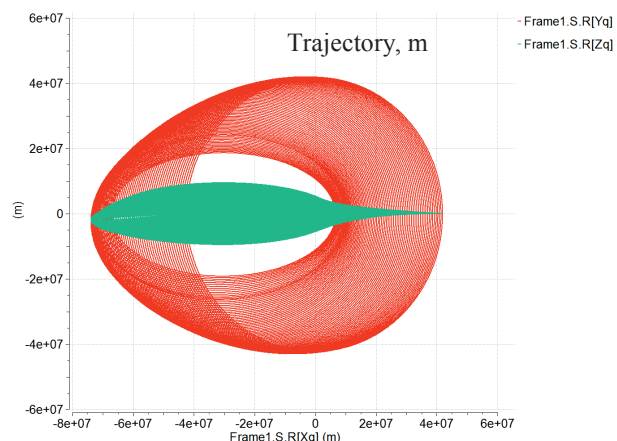
Figure 2. Orbit transfer optimised in operations
