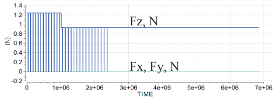
Figure 3. Thrust level (drop to zero in eclipse)
