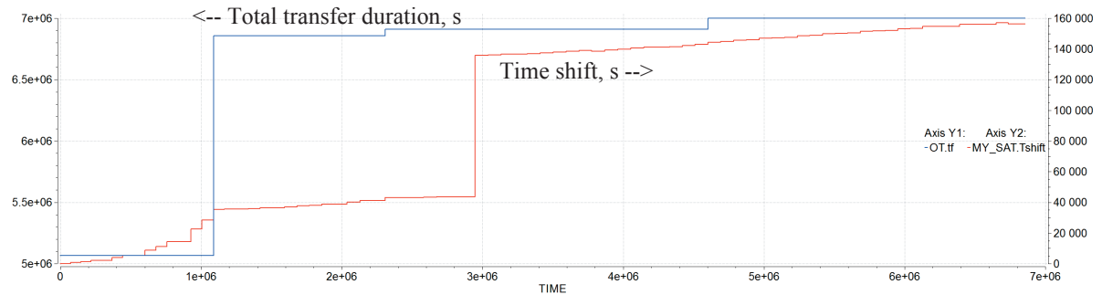
Figure 9. Total transfer duration each time the Optimiser is called and time shift synchronization at perigee
