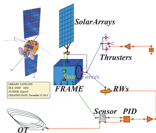
Figure 1. System model under EcosimPro ESPSS
