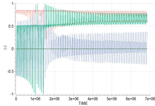
Figure 7. Quaternion of satellite attitude
