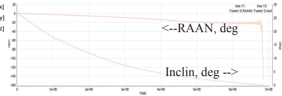
Figure 4. RAAN and inclination evolutions
