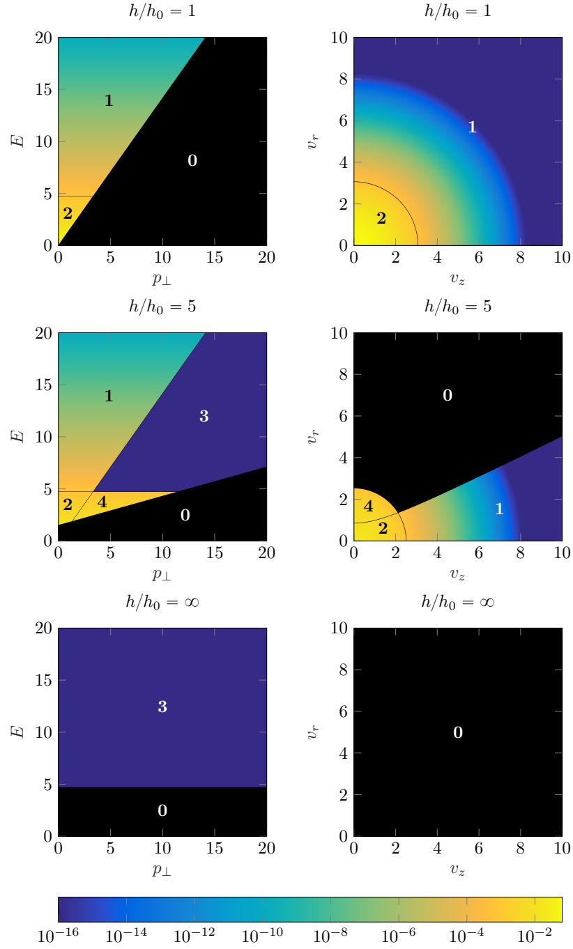
Figure 5. Evolution of the electron velocity distribution function \bar{f}_e at different values of h , for \chi = 0.02 , \mu \rightarrow \infty and \alpha = 1 . Plots on the left show the (E, p_{\perp}) plane; those on the right the (v_z, v_r) plane at the plume axis ( r = 0 ). The color map shows the magnitude of \bar{f}_e . The different regions of phase space are labeled according to the enumeration of Section A.
