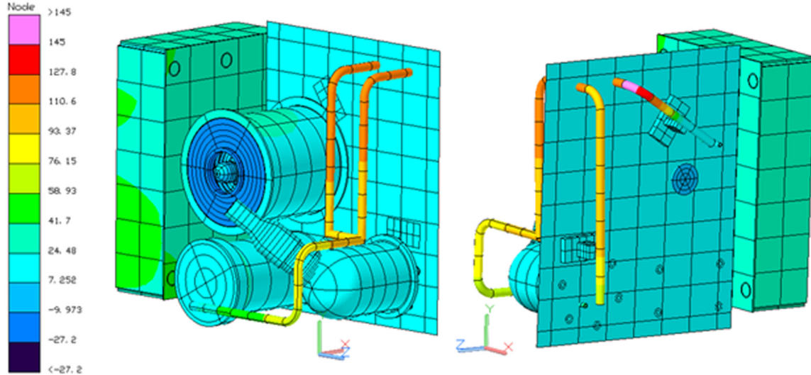
Figure 8. Temperature (in degrees Celsius) of propulsion components at a representative time during the pre-thrust period with \beta=90^\circ .
