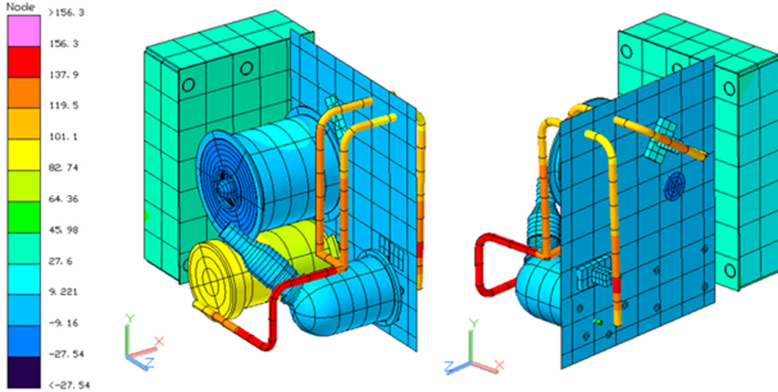
Figure 7. Temperature (in degrees Celsius) of propulsion components at a representative time during the pre-thrust period with \beta=0^\circ .
