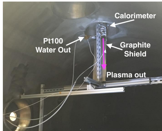
Fig. 5 Calorimeter installation
