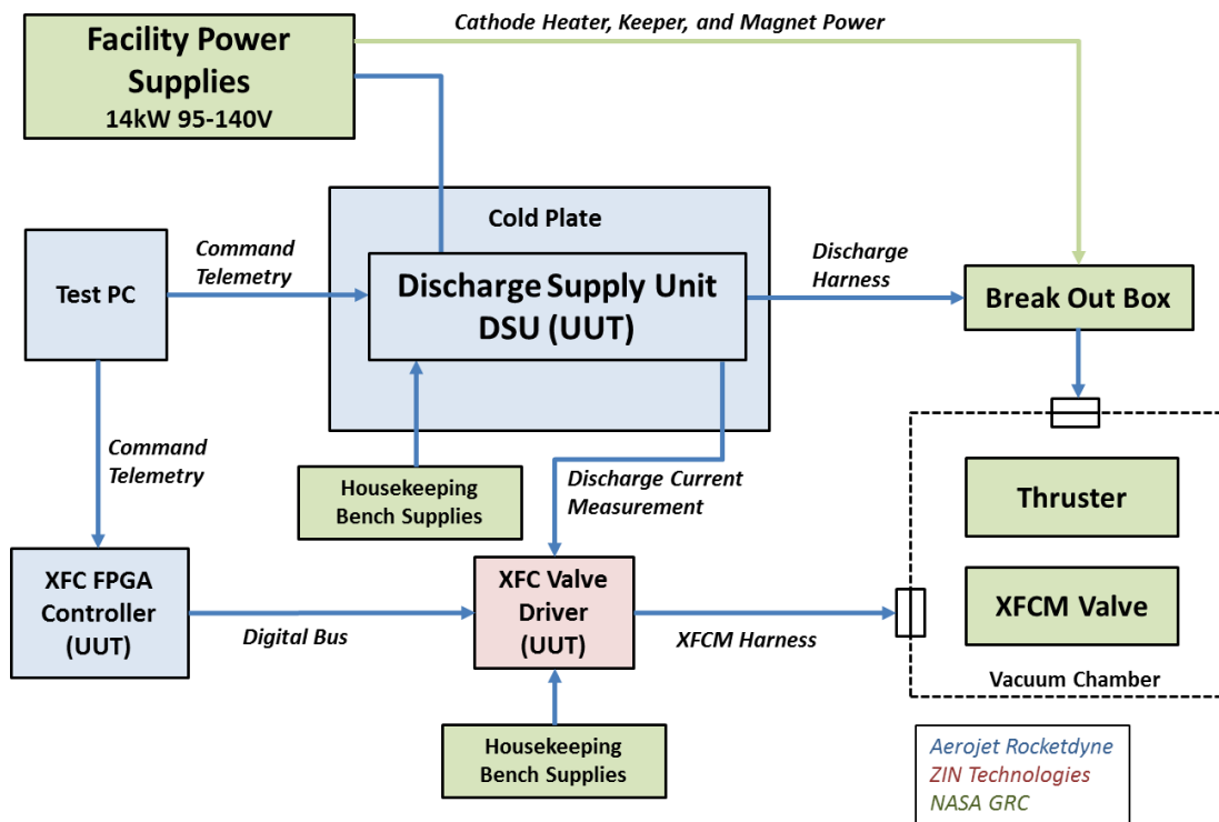
Figure 13. Test Setup
