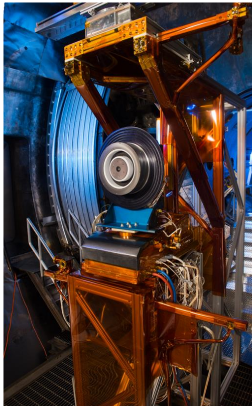
Figure 7. High-power thruster stand installed in VF-6 with the TDU-3 Hall thruster.
