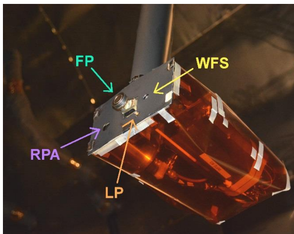
Figure 8. The VF-6 plasma diagnostic probe package.
