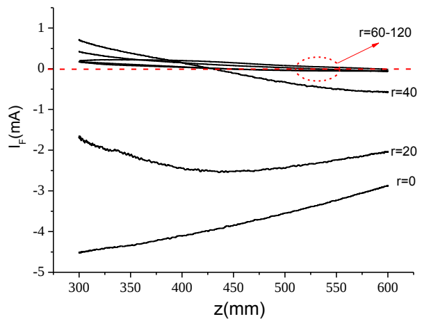
(f) Axial current-distribution ( B_a = 127 mT)
