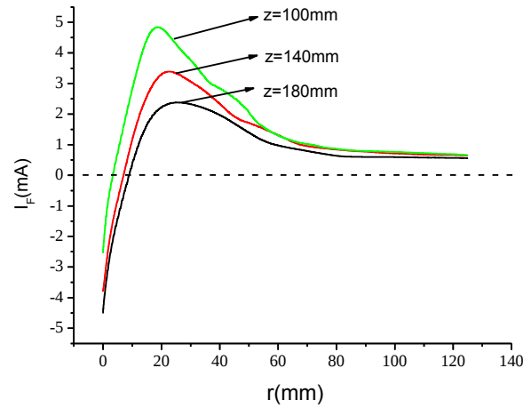
(a) Radial current distribution ( B_a = 64 mT)
