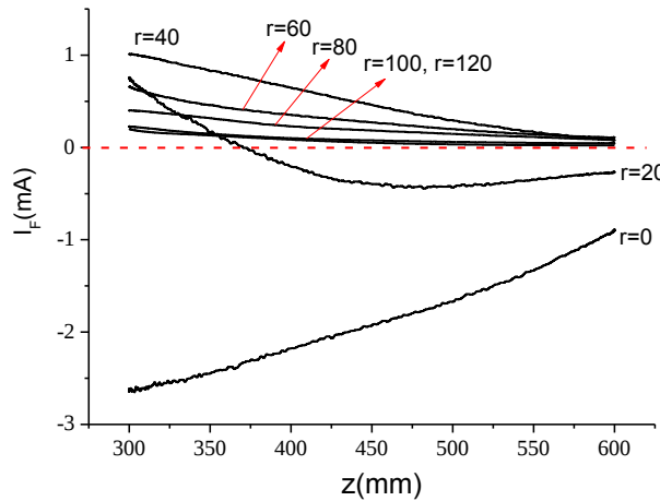
(e) Axial current-distribution ( B_a = 64 mT)
