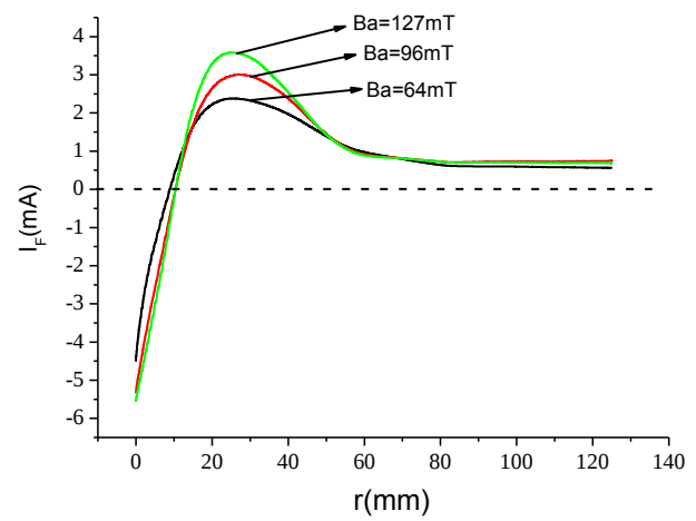
(d) Comparison of radial current distribution under 64 mT, 96 mT and 127 mT ( z = 180 mm)
