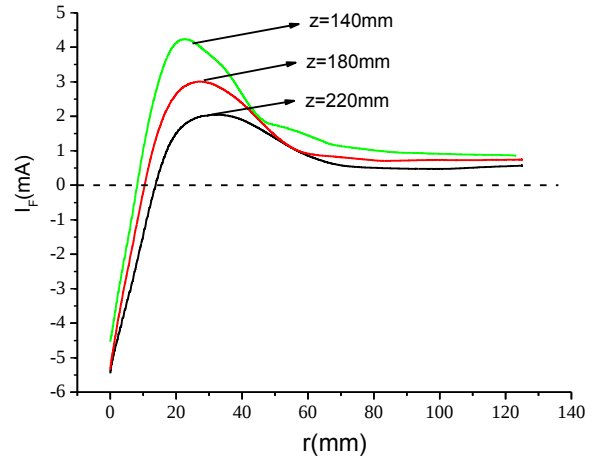
(b) Radial current distribution ( B_a = 96 mT)
