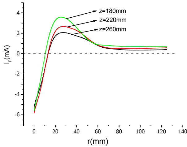
(c) Radial current distribution ( B_a = 127 mT)
