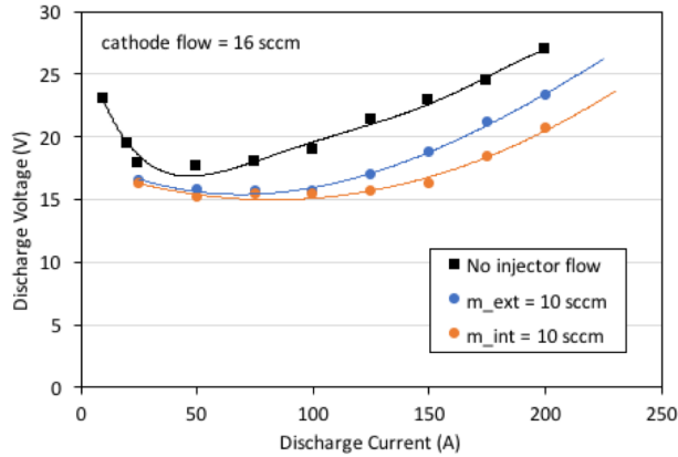
Figure 7. Discharge voltage versus current at 16 sccm xenon flow showing the effect of flow through the two injector systems.
