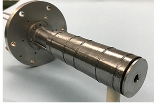
Figure 9. LaB 6 cathode with the 3.2cm dia. orifice plate.
