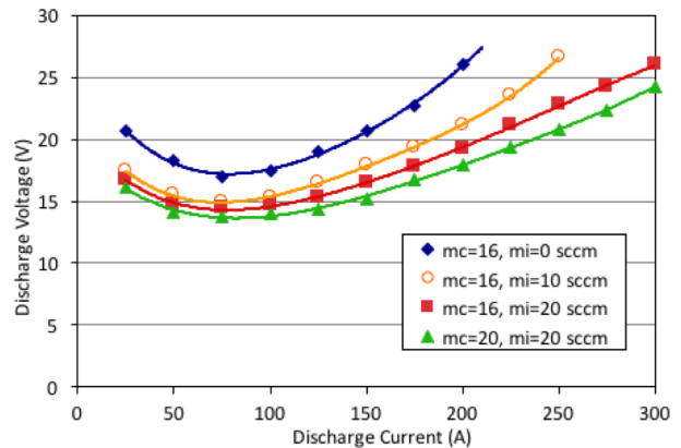
Figure 8. Discharge voltage versus current showing the effect of external gas injection. Discharge currents of up to 300 A were achieved with sufficient external injection.
