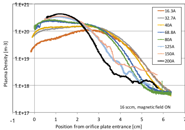
Figure 11. Internal plasma density profiles at various currents for 16 sccm cathode flow conditions.
