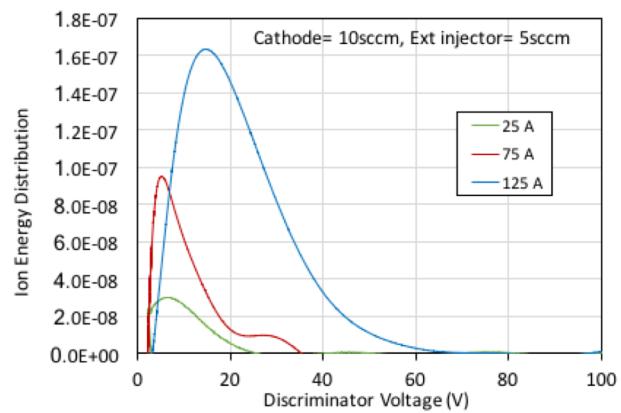
Figure 12. Ion energy distribution at three discharge currents for xenon flow of 10 sccm through the cathode and 5 sccm through the external injector. 30 to >60 V energetic ions are observed at higher currents.
