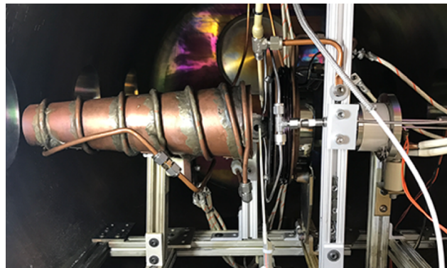
Figure 5a. High power test facility setup with gas injectors.
