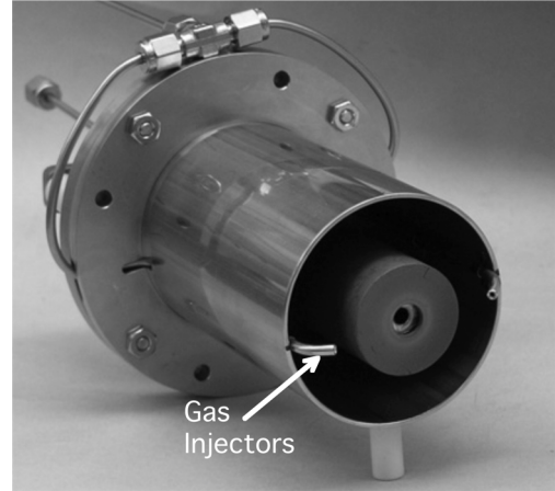
Figure 6. Lanthanum hexaboride hollow cathode assembly with cathode-plume gas injectors.
