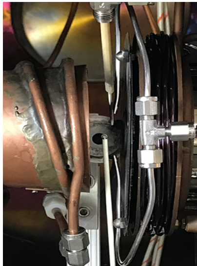
Figure 5b. Close-up photo of RPA, external gas injectors and two probes used for cathode-plume studies.
