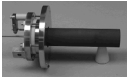
Figure 2. The laboratory-model 2-cm-dia. LaB 6 hollow cathode.
