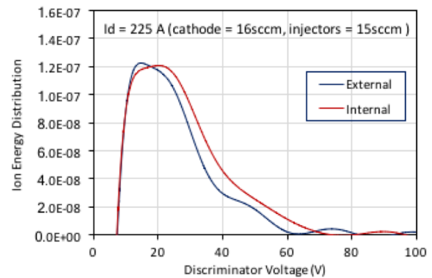
Figure 13. Comparison of ion energy distribution at 225 A of discharge current for 16 sccm flow through the cathode and 15 sccm through the external injector or the internal injector.
