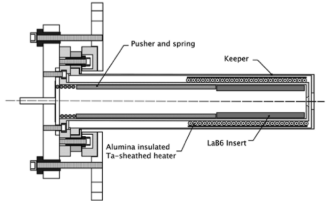
Figure 1. Schematic of the 2-cm-dia. LaB 6 hollow cathode.
