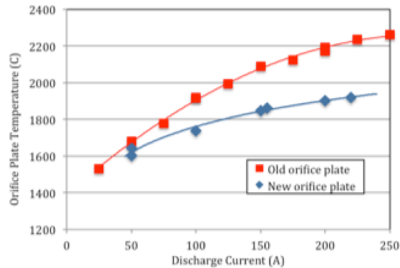
Figure 4. Orifice plate temperature versus discharge current for two outside diameters of the cathode orifice plate.
